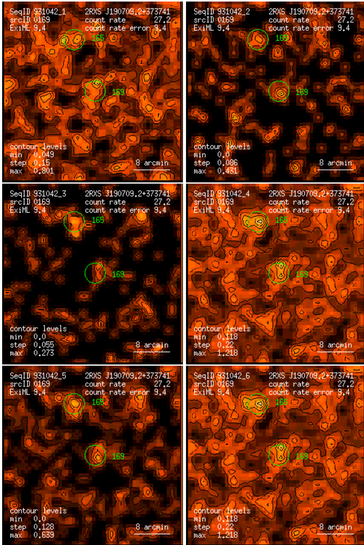
Figure 169: RASS 931042: detection 0169: band rate images, Gaussian filter: (1) PSPC channels 11 – 41, (2) 52 – 90, (3) 91 – 201, (4) 11 – 235, (5) 52 – 201, (6) 11 – 201. Broad band rates in counts/ks. Band rate contour levels in counts/ks/arcmin 2 .
