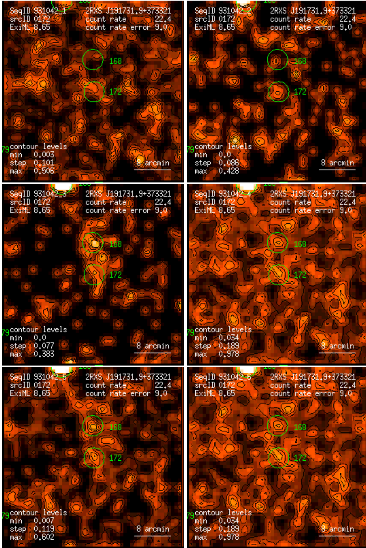
Figure 172: RASS 931042: detection 0172: band rate images, Gaussian filter: (1) PSPC channels 11 – 41, (2) 52 – 90, (3) 91 – 201, (4) 11 – 235, (5) 52 – 201, (6) 11 – 201. Broad band rates in counts/ks. Band rate contour levels in counts/ks/arcmin 2 .
