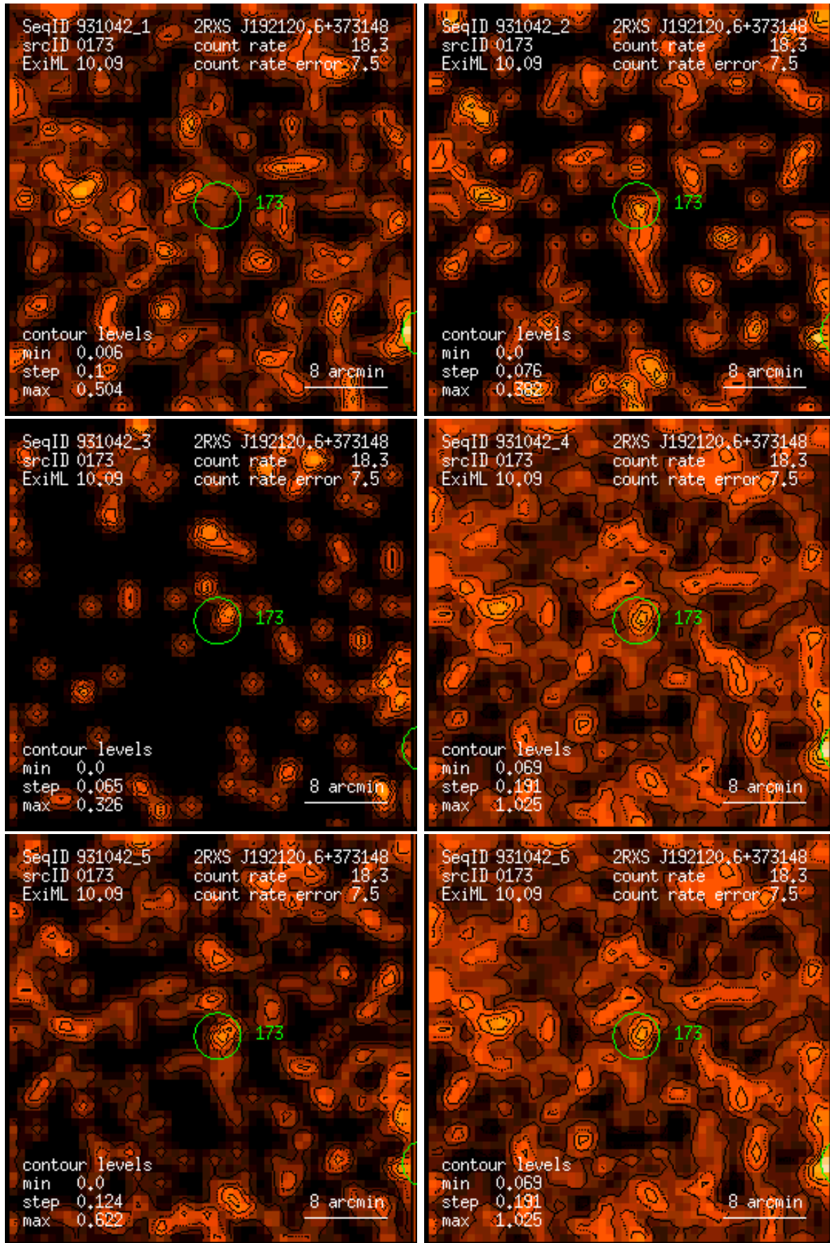
Figure 173: RASS 931042: detection 0173: band rate images, Gaussian filter: (1) PSPC channels 11 – 41, (2) 52 – 90, (3) 91 – 201, (4) 11 – 235, (5) 52 – 201, (6) 11 – 201. Broad band rates in counts/ks. Band rate contour levels in counts/ks/arcmin 2 .
