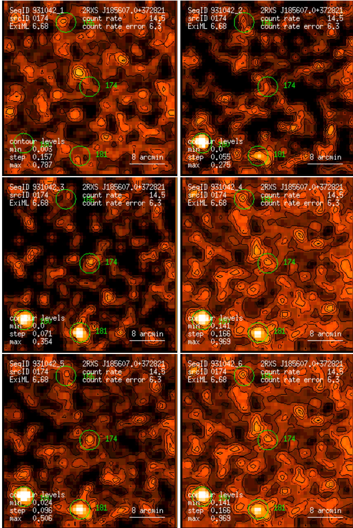
Figure 174: RASS 931042: detection 0174: band rate images, Gaussian filter: (1) PSPC channels 11 – 41, (2) 52 – 90, (3) 91 – 201, (4) 11 – 235, (5) 52 – 201, (6) 11 – 201. Broad band rates in counts/ks. Band rate contour levels in counts/ks/arcmin 2 .
