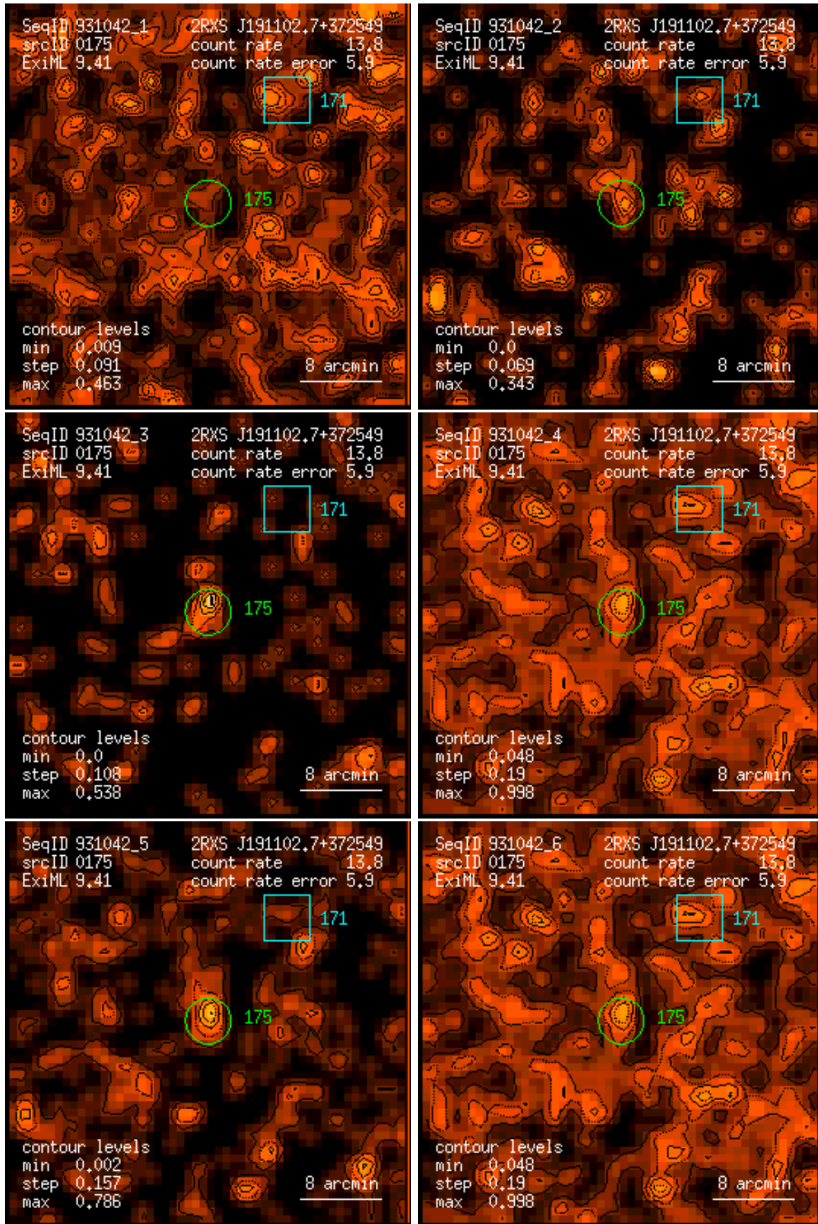
Figure 175: RASS 931042: detection 0175: band rate images, Gaussian filter: (1) PSPC channels 11 – 41, (2) 52 – 90, (3) 91 – 201, (4) 11 – 235, (5) 52 – 201, (6) 11 – 201. Broad band rates in counts/ks. Band rate contour levels in counts/ks/arcmin 2 .
