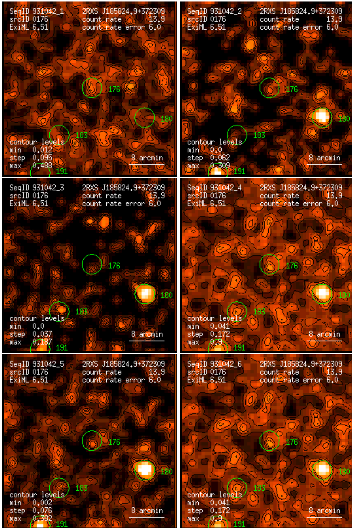
Figure 176: RASS 931042: detection 0176: band rate images, Gaussian filter: (1) PSPC channels 11 – 41, (2) 52 – 90, (3) 91 – 201, (4) 11 – 235, (5) 52 – 201, (6) 11 – 201. Broad band rates in counts/ks. Band rate contour levels in counts/ks/arcmin 2 .
