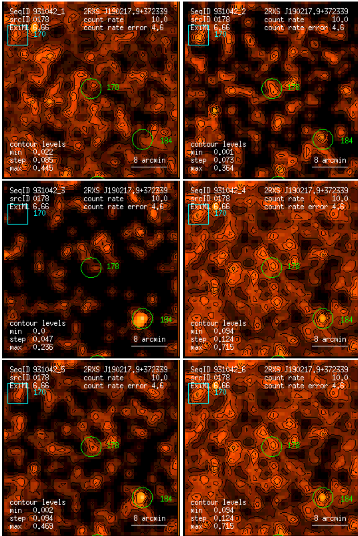
Figure 178: RASS 931042: detection 0178: band rate images, Gaussian filter: (1) PSPC channels 11 – 41, (2) 52 – 90, (3) 91 – 201, (4) 11 – 235, (5) 52 – 201, (6) 11 – 201. Broad band rates in counts/ks. Band rate contour levels in counts/ks/arcmin 2 .
