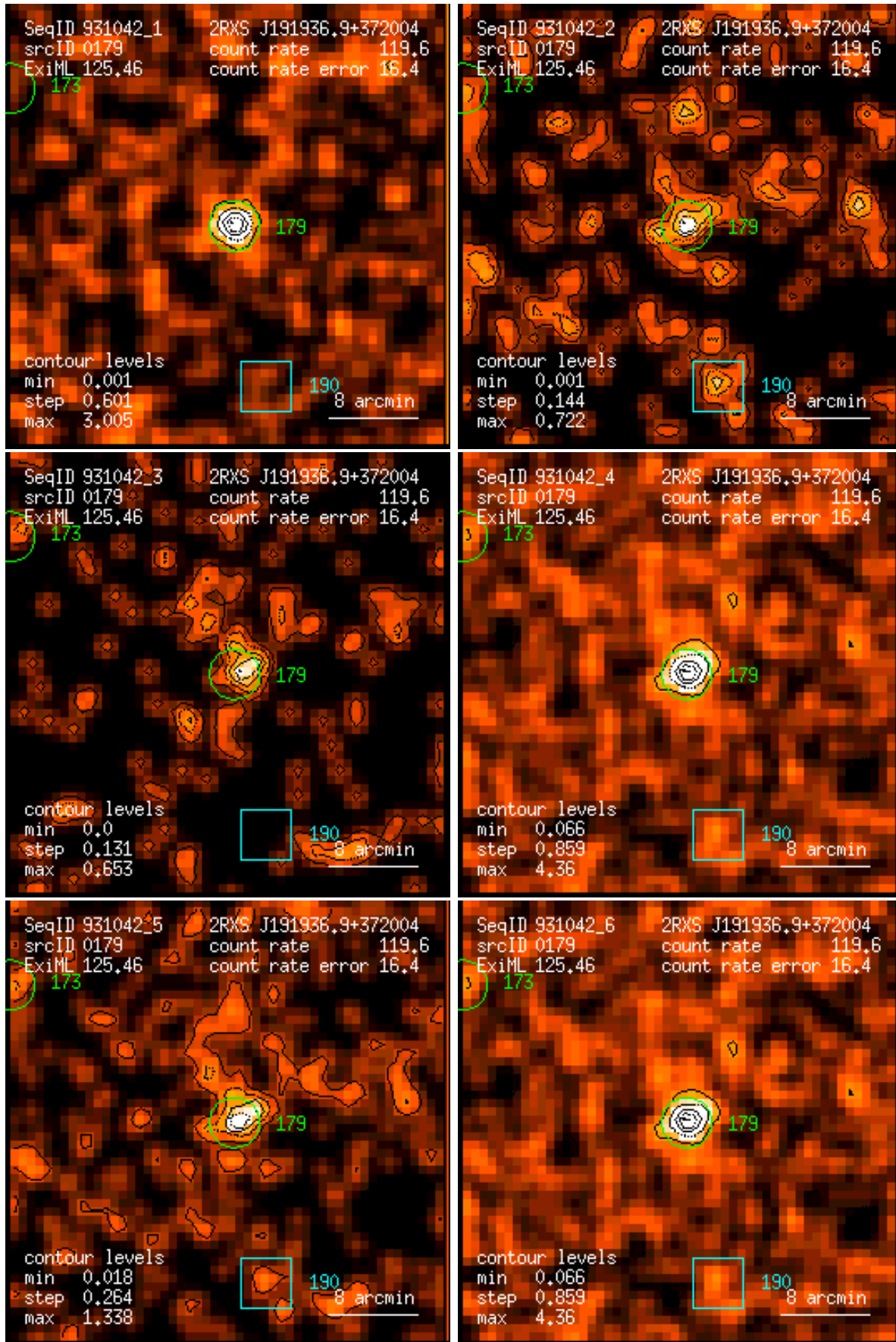
Figure 179: RASS 931042: detection 0179: band rate images, Gaussian filter: (1) PSPC channels 11 – 41, (2) 52 – 90, (3) 91 – 201, (4) 11 – 235, (5) 52 – 201, (6) 11 – 201. Broad band rates in counts/ks. Band rate contour levels in counts/ks/arcmin 2 .
