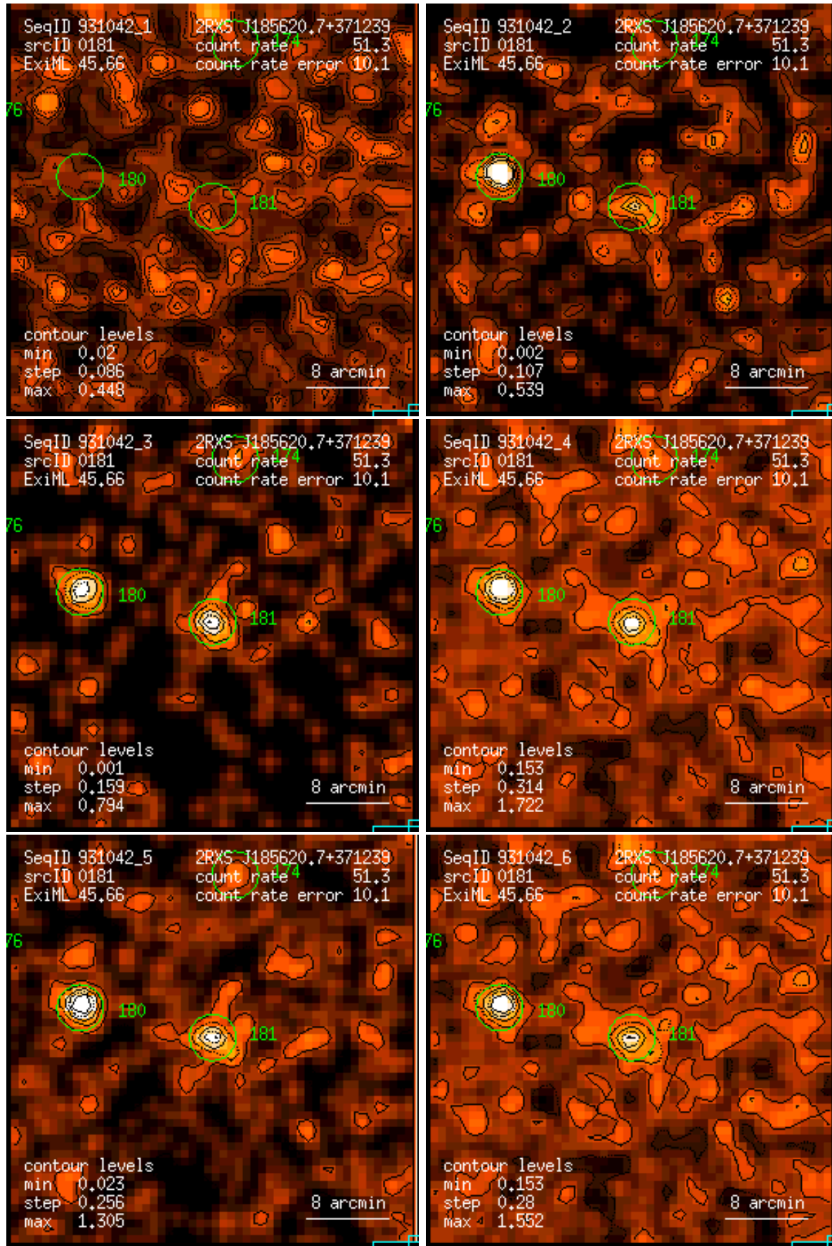
Figure 181: RASS 931042: detection 0181: band rate images, Gaussian filter: (1) PSPC channels 11 – 41, (2) 52 – 90, (3) 91 – 201, (4) 11 – 235, (5) 52 – 201, (6) 11 – 201. Broad band rates in counts/ks. Band rate contour levels in counts/ks/arcmin 2 .
