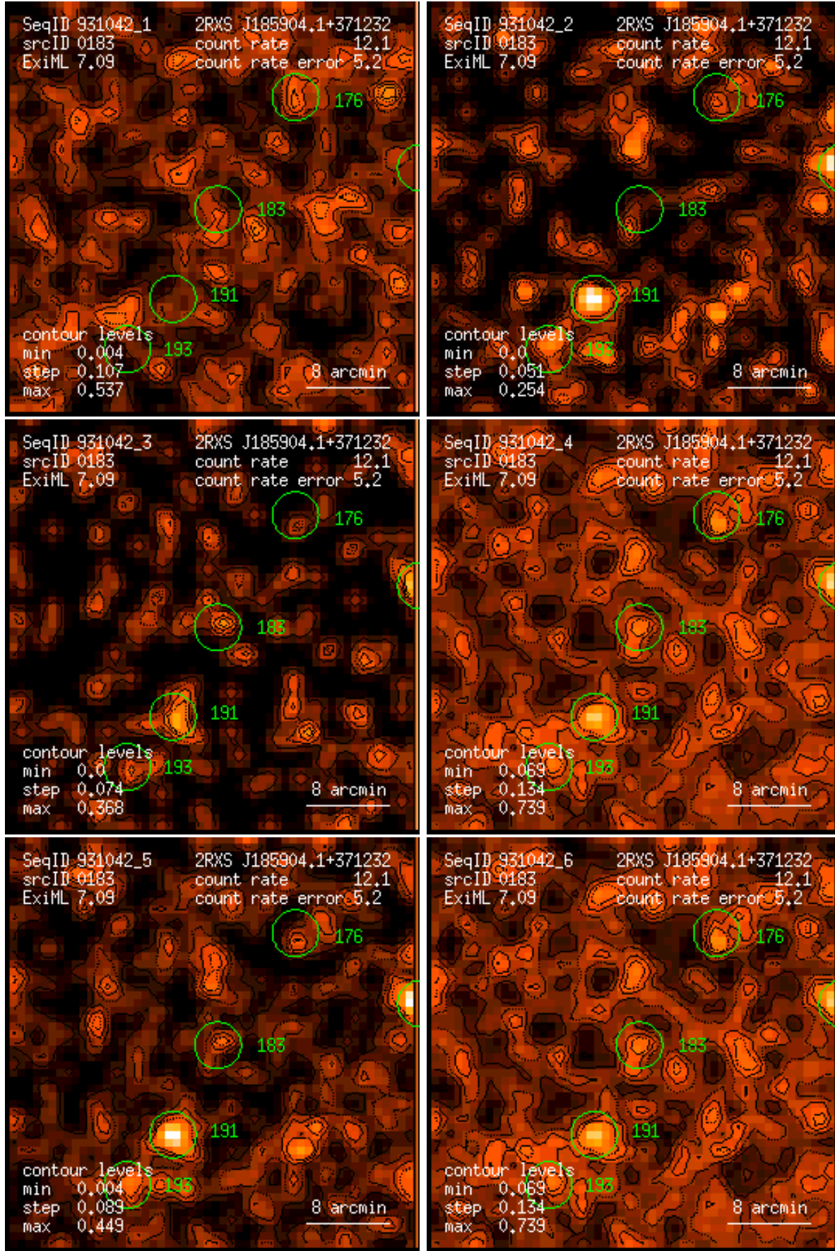
Figure 183: RASS 931042: detection 0183: band rate images, Gaussian filter: (1) PSPC channels 11 – 41, (2) 52 – 90, (3) 91 – 201, (4) 11 – 235, (5) 52 – 201, (6) 11 – 201. Broad band rates in counts/ks. Band rate contour levels in counts/ks/arcmin 2 .
