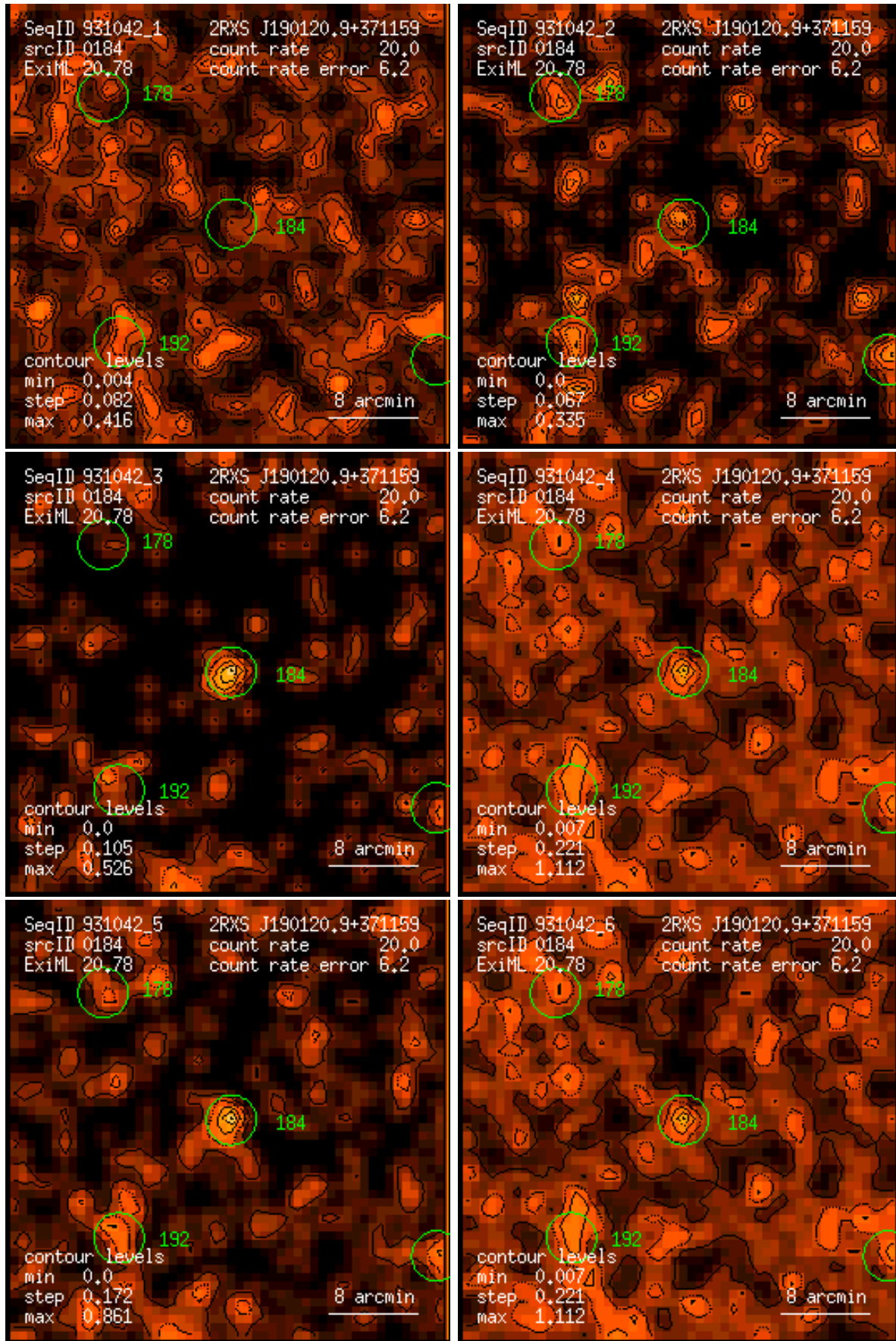
Figure 184: RASS 931042: detection 0184: band rate images, Gaussian filter: (1) PSPC channels 11 – 41, (2) 52 – 90, (3) 91 – 201, (4) 11 – 235, (5) 52 – 201, (6) 11 – 201. Broad band rates in counts/ks. Band rate contour levels in counts/ks/arcmin 2 .
