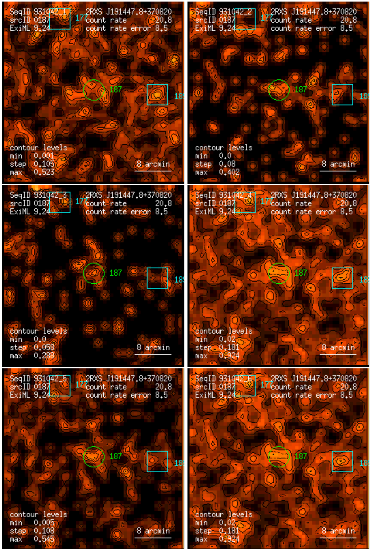
Figure 187: RASS 931042: detection 0187: band rate images, Gaussian filter: (1) PSPC channels 11 – 41, (2) 52 – 90, (3) 91 – 201, (4) 11 – 235, (5) 52 – 201, (6) 11 – 201. Broad band rates in counts/ks. Band rate contour levels in counts/ks/arcmin 2 .
