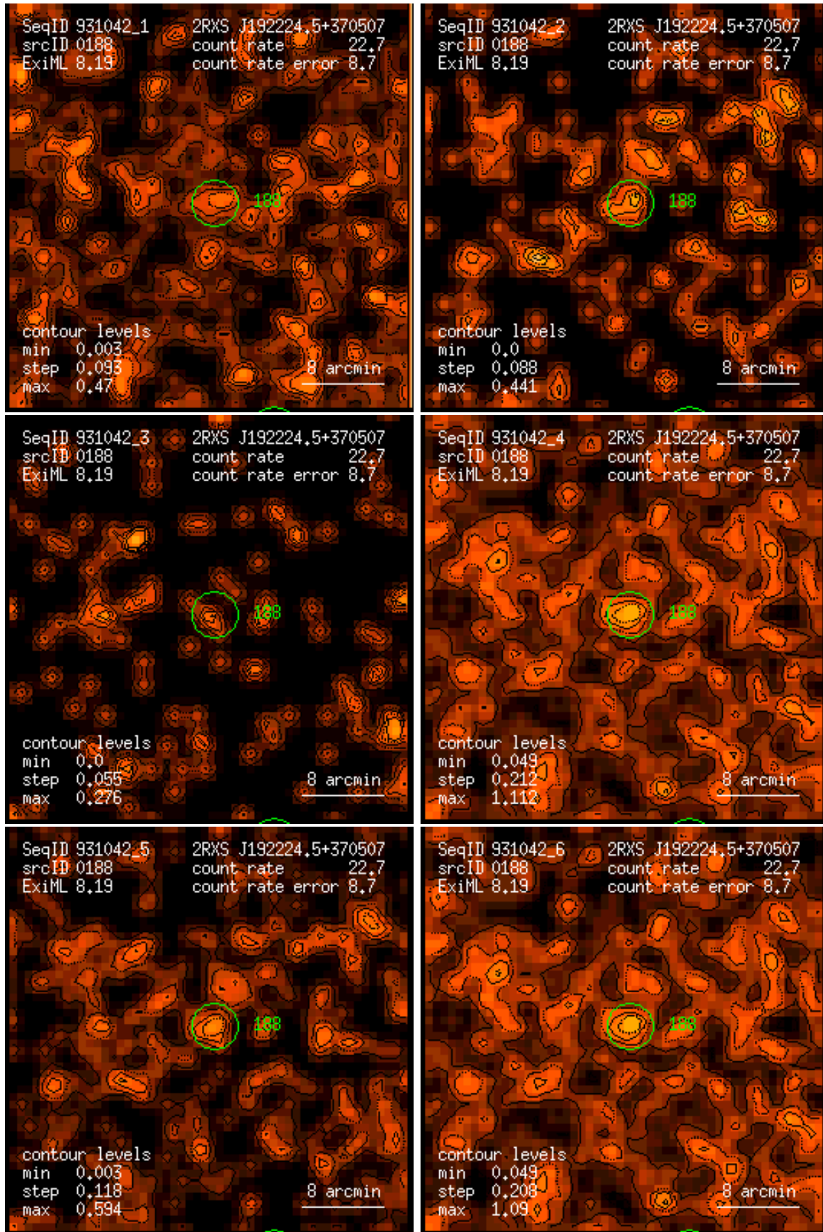
Figure 188: RASS 931042: detection 0188: band rate images, Gaussian filter: (1) PSPC channels 11 – 41, (2) 52 – 90, (3) 91 – 201, (4) 11 – 235, (5) 52 – 201, (6) 11 – 201. Broad band rates in counts/ks. Band rate contour levels in counts/ks/arcmin 2 .
