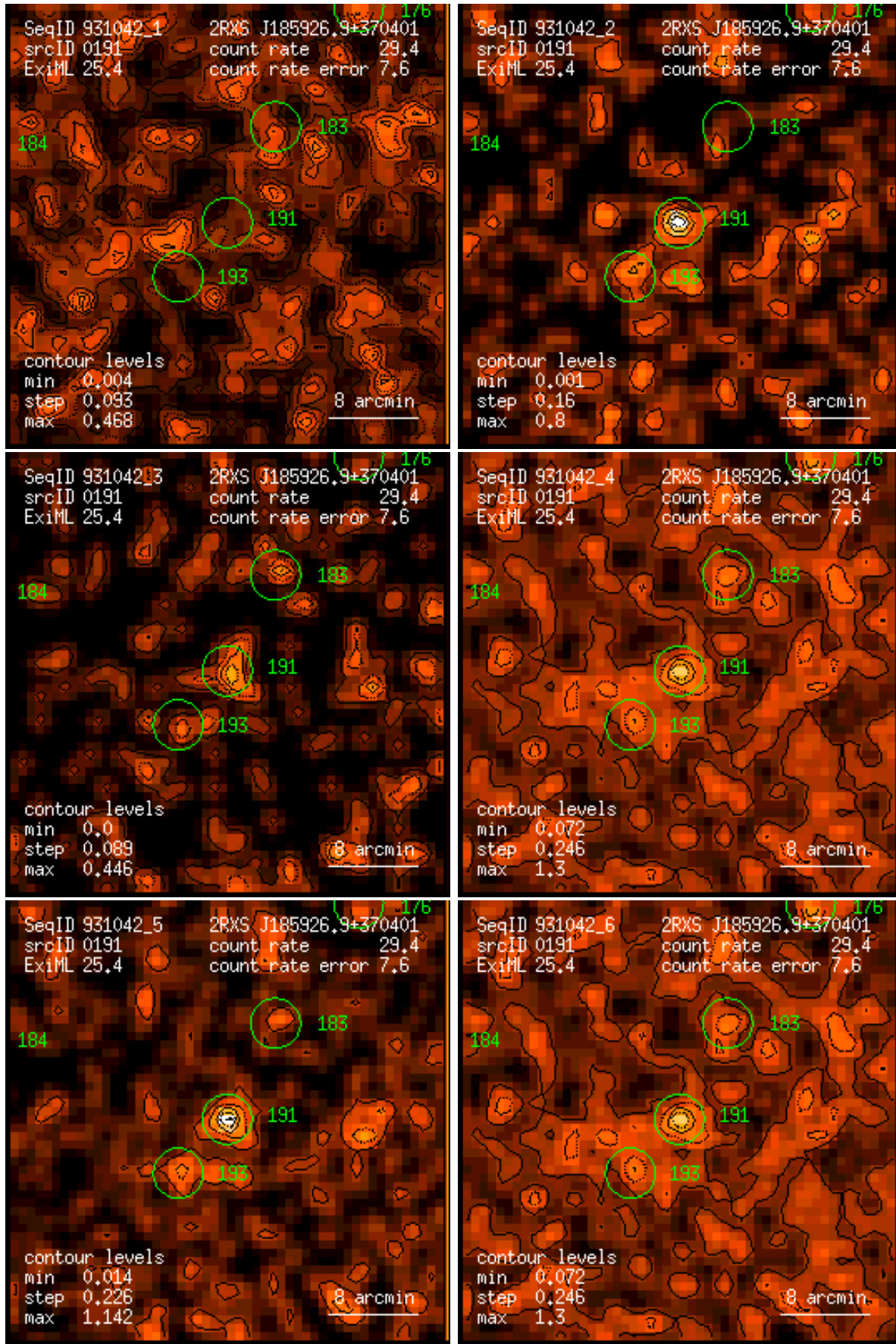
Figure 191: RASS 931042: detection 0191: band rate images, Gaussian filter: (1) PSPC channels 11 – 41, (2) 52 – 90, (3) 91 – 201, (4) 11 – 235, (5) 52 – 201, (6) 11 – 201. Broad band rates in counts/ks. Band rate contour levels in counts/ks/arcmin 2 .
