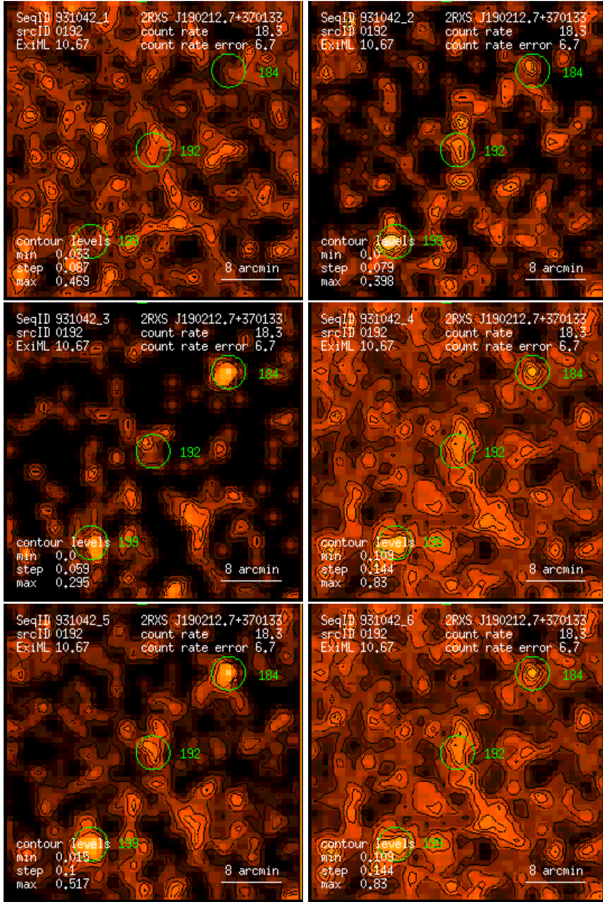
Figure 192: RASS 931042: detection 0192: band rate images, Gaussian filter: (1) PSPC channels 11 – 41, (2) 52 – 90, (3) 91 – 201, (4) 11 – 235, (5) 52 – 201, (6) 11 – 201. Broad band rates in counts/ks. Band rate contour levels in counts/ks/arcmin 2 .
