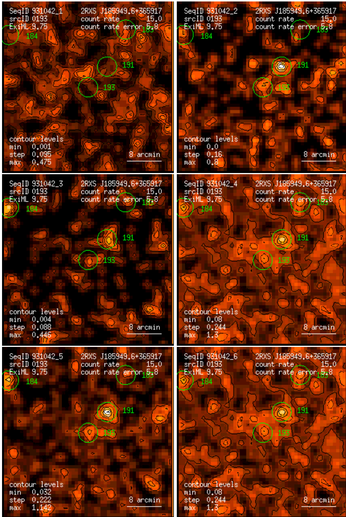
Figure 193: RASS 931042: detection 0193: band rate images, Gaussian filter: (1) PSPC channels 11 – 41, (2) 52 – 90, (3) 91 – 201, (4) 11 – 235, (5) 52 – 201, (6) 11 – 201. Broad band rates in counts/ks. Band rate contour levels in counts/ks/arcmin 2 .
