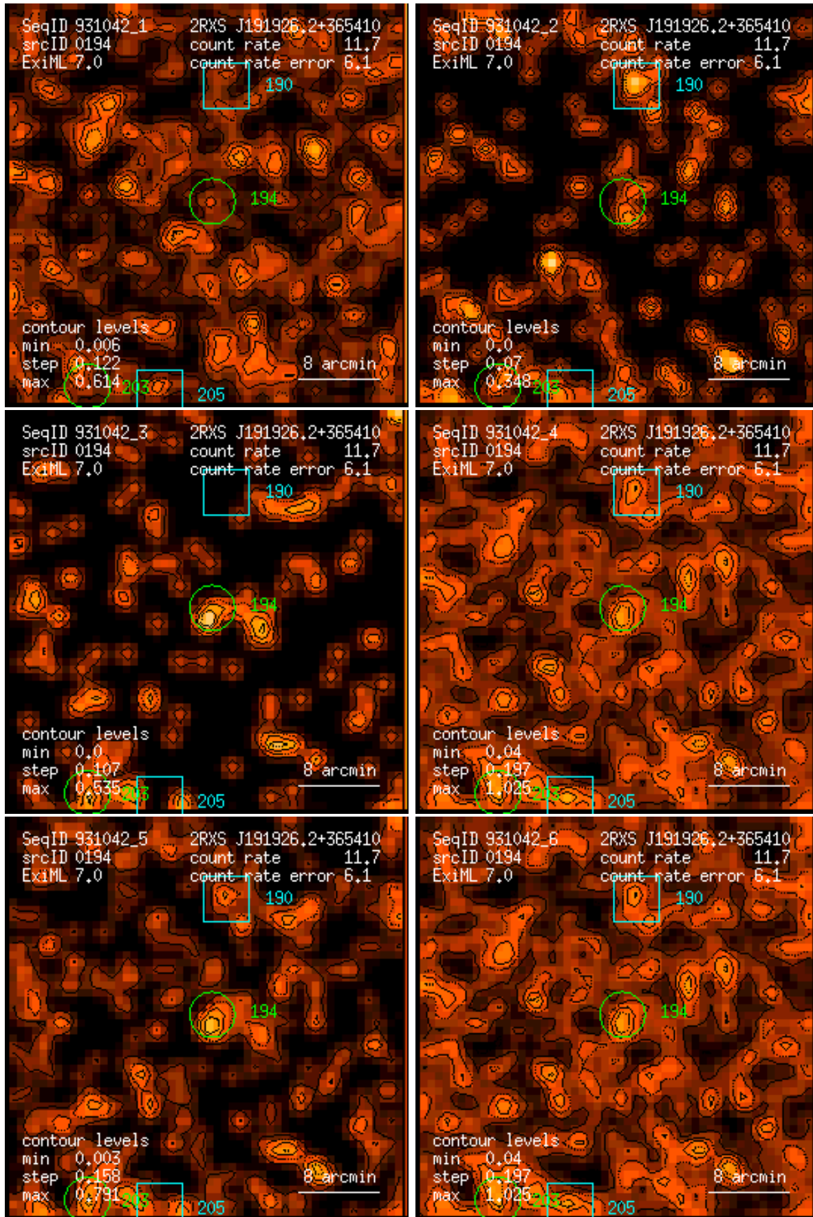
Figure 194: RASS 931042: detection 0194: band rate images, Gaussian filter: (1) PSPC channels 11 – 41, (2) 52 – 90, (3) 91 – 201, (4) 11 – 235, (5) 52 – 201, (6) 11 – 201. Broad band rates in counts/ks. Band rate contour levels in counts/ks/arcmin 2 .
