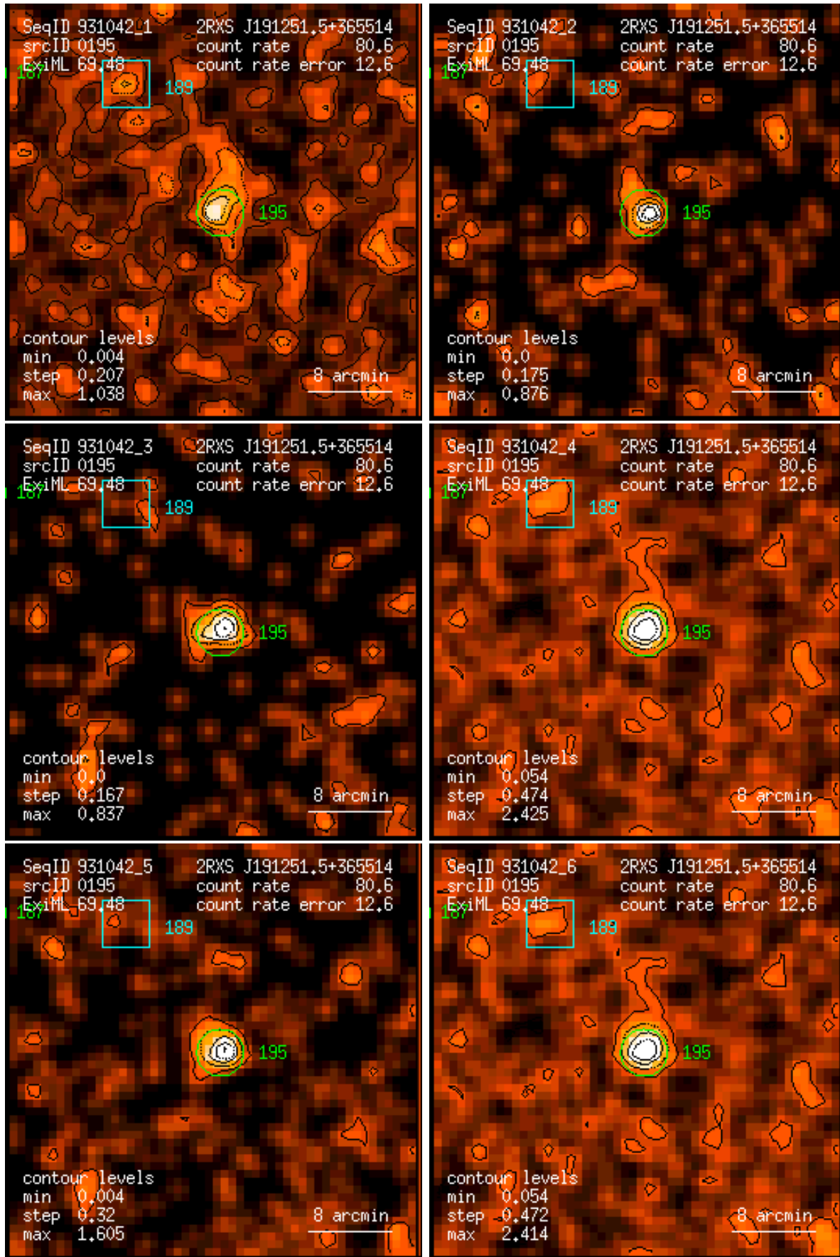
Figure 195: RASS 931042: detection 0195: band rate images, Gaussian filter: (1) PSPC channels 11 – 41, (2) 52 – 90, (3) 91 – 201, (4) 11 – 235, (5) 52 – 201, (6) 11 – 201. Broad band rates in counts/ks. Band rate contour levels in counts/ks/arcmin 2 .
