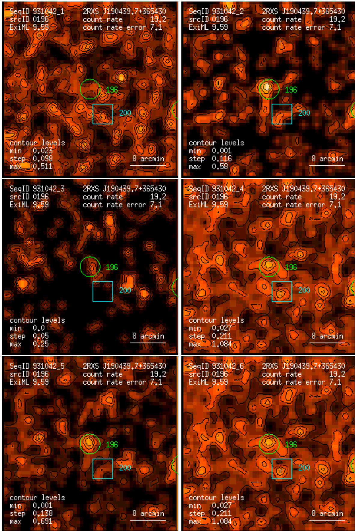
Figure 196: RASS 931042: detection 0196: band rate images, Gaussian filter: (1) PSPC channels 11 – 41, (2) 52 – 90, (3) 91 – 201, (4) 11 – 235, (5) 52 – 201, (6) 11 – 201. Broad band rates in counts/ks. Band rate contour levels in counts/ks/arcmin 2 .
