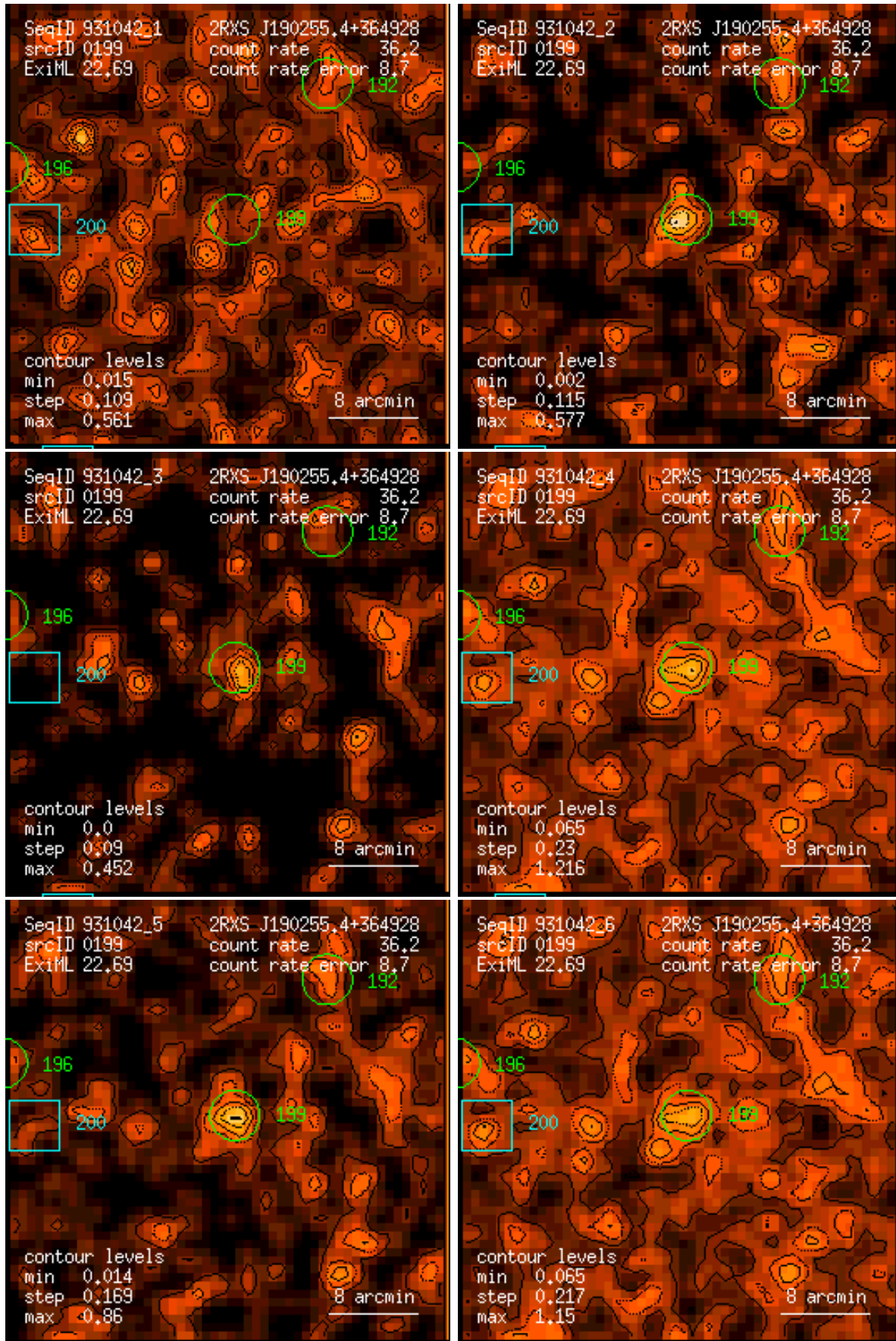
Figure 199: RASS 931042: detection 0199: band rate images, Gaussian filter: (1) PSPC channels 11 – 41, (2) 52 – 90, (3) 91 – 201, (4) 11 – 235, (5) 52 – 201, (6) 11 – 201. Broad band rates in counts/ks. Band rate contour levels in counts/ks/arcmin 2 .
