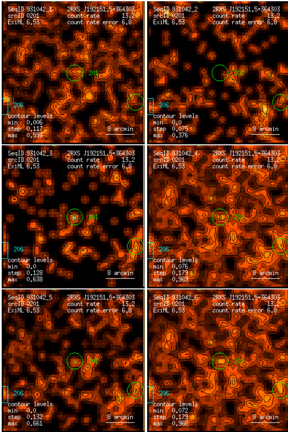
Figure 201: RASS 931042: detection 0201: band rate images, Gaussian filter: (1) PSPC channels 11 – 41, (2) 52 – 90, (3) 91 – 201, (4) 11 – 235, (5) 52 – 201, (6) 11 – 201. Broad band rates in counts/ks. Band rate contour levels in counts/ks/arcmin 2 .
