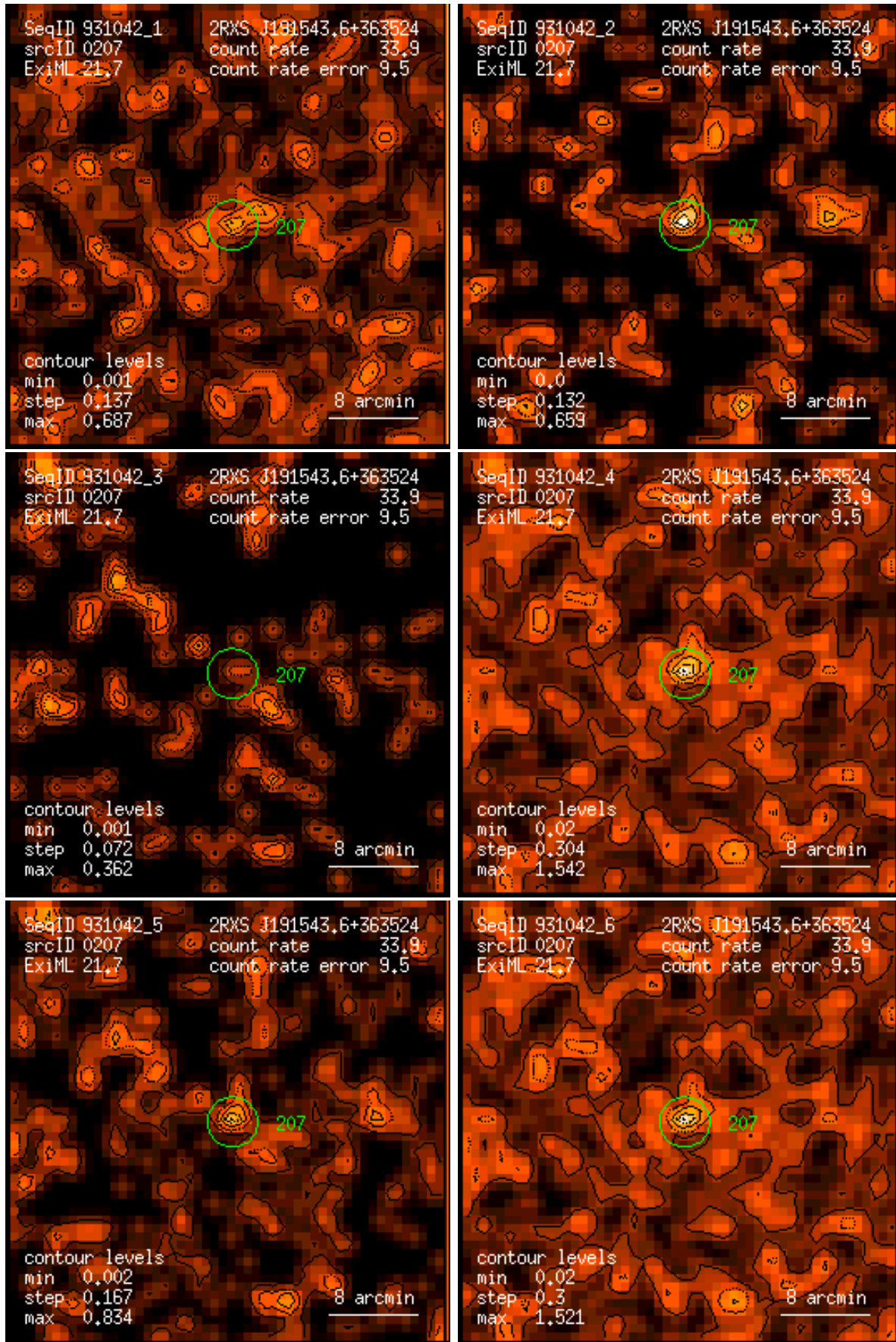
Figure 207: RASS 931042: detection 0207: band rate images, Gaussian filter: (1) PSPC channels 11 – 41, (2) 52 – 90, (3) 91 – 201, (4) 11 – 235, (5) 52 – 201, (6) 11 – 201. Broad band rates in counts/ks. Band rate contour levels in counts/ks/arcmin 2 .
