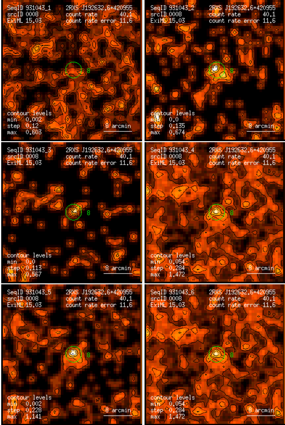
Figure 8: RASS 931043: detection 0008: band rate images, Gaussian filter: (1) PSPC channels 11 – 41, (2) 52 – 90, (3) 91 – 201, (4) 11 – 235, (5) 52 – 201, (6) 11 – 201. Broad band rates in counts/ks. Band rate contour levels in counts/ks/arcmin 2 .
