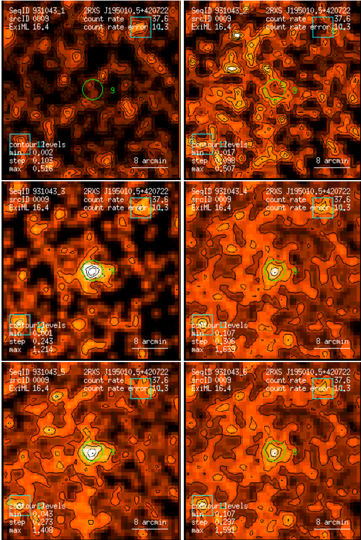
Figure 9: RASS 931043: detection 0009: band rate images, Gaussian filter: (1) PSPC channels 11 – 41, (2) 52 – 90, (3) 91 – 201, (4) 11 – 235, (5) 52 – 201, (6) 11 – 201. Broad band rates in counts/ks. Band rate contour levels in counts/ks/arcmin 2 .
