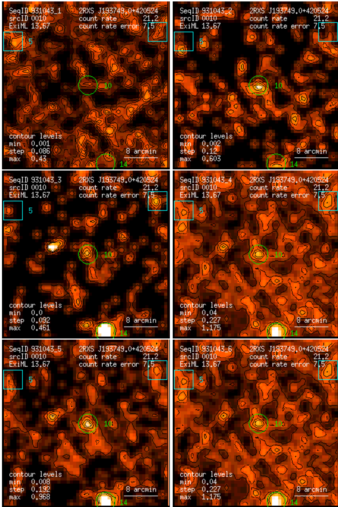
Figure 10: RASS 931043: detection 0010: band rate images, Gaussian filter: (1) PSPC channels 11 – 41, (2) 52 – 90, (3) 91 – 201, (4) 11 – 235, (5) 52 – 201, (6) 11 – 201. Broad band rates in counts/ks. Band rate contour levels in counts/ks/arcmin 2 .
