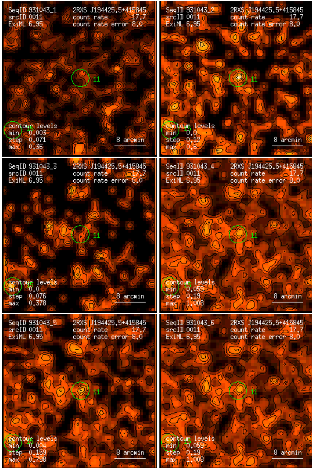
Figure 11: RASS 931043: detection 0011: band rate images, Gaussian filter: (1) PSPC channels 11 – 41, (2) 52 – 90, (3) 91 – 201, (4) 11 – 235, (5) 52 – 201, (6) 11 – 201. Broad band rates in counts/ks. Band rate contour levels in counts/ks/arcmin 2 .
