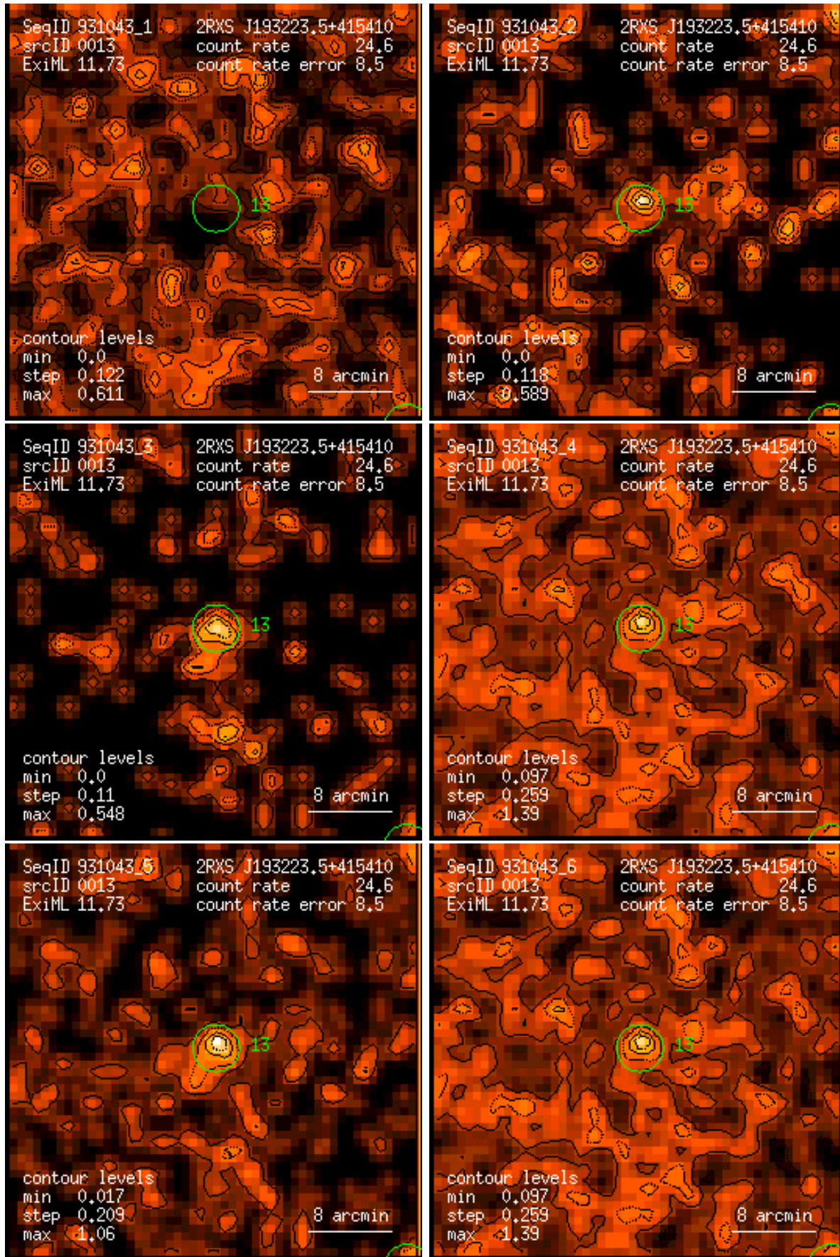
Figure 13: RASS 931043: detection 0013: band rate images, Gaussian filter: (1) PSPC channels 11 – 41, (2) 52 – 90, (3) 91 – 201, (4) 11 – 235, (5) 52 – 201, (6) 11 – 201. Broad band rates in counts/ks. Band rate contour levels in counts/ks/arcmin 2 .
