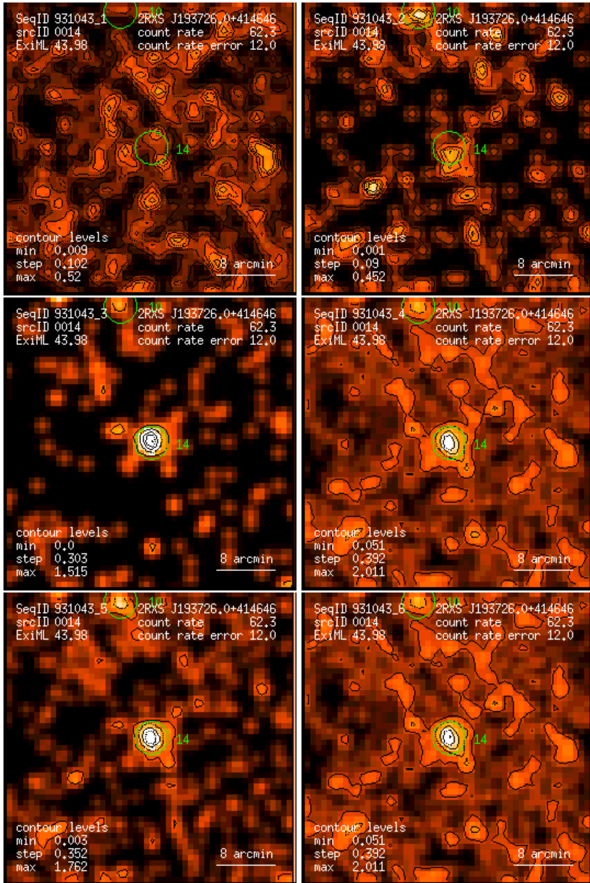
Figure 14: RASS 931043: detection 0014: band rate images, Gaussian filter: (1) PSPC channels 11 – 41, (2) 52 – 90, (3) 91 – 201, (4) 11 – 235, (5) 52 – 201, (6) 11 – 201. Broad band rates in counts/ks. Band rate contour levels in counts/ks/arcmin 2 .
