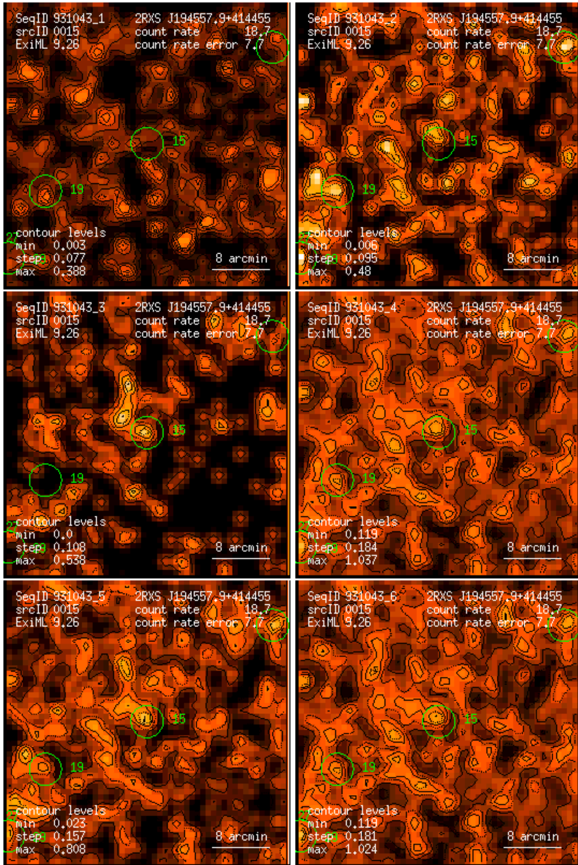
Figure 15: RASS 931043: detection 0015: band rate images, Gaussian filter: (1) PSPC channels 11 – 41, (2) 52 – 90, (3) 91 – 201, (4) 11 – 235, (5) 52 – 201, (6) 11 – 201. Broad band rates in counts/ks. Band rate contour levels in counts/ks/arcmin 2 .
