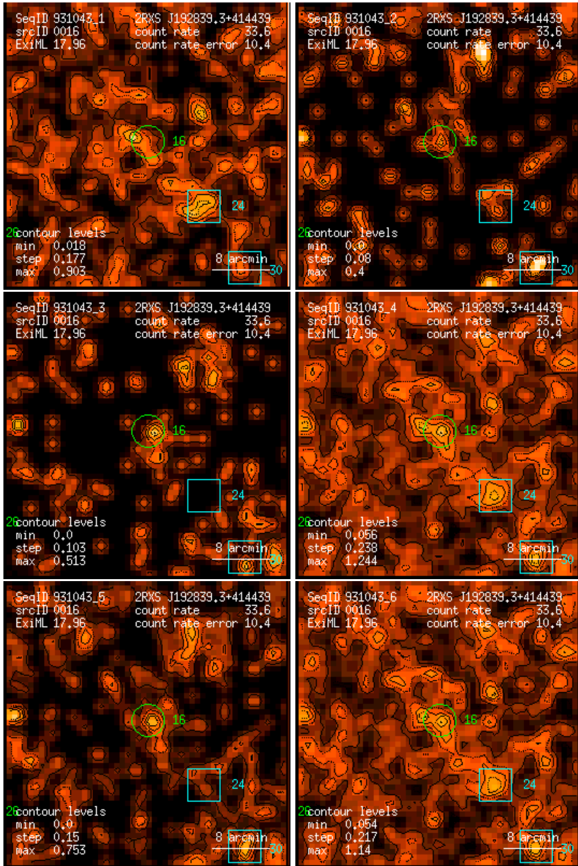
Figure 16: RASS 931043: detection 0016: band rate images, Gaussian filter: (1) PSPC channels 11 – 41, (2) 52 – 90, (3) 91 – 201, (4) 11 – 235, (5) 52 – 201, (6) 11 – 201. Broad band rates in counts/ks. Band rate contour levels in counts/ks/arcmin 2 .
