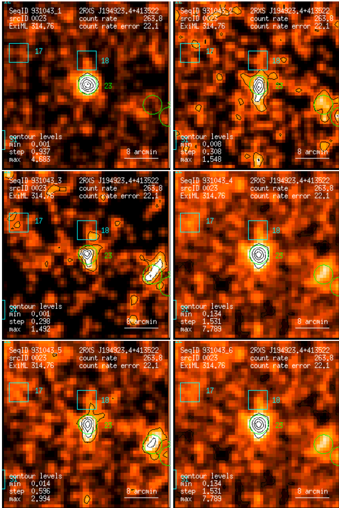
Figure 23: RASS 931043: detection 0023: band rate images, Gaussian filter: (1) PSPC channels 11 – 41, (2) 52 – 90, (3) 91 – 201, (4) 11 – 235, (5) 52 – 201, (6) 11 – 201. Broad band rates in counts/ks. Band rate contour levels in counts/ks/arcmin 2 .
