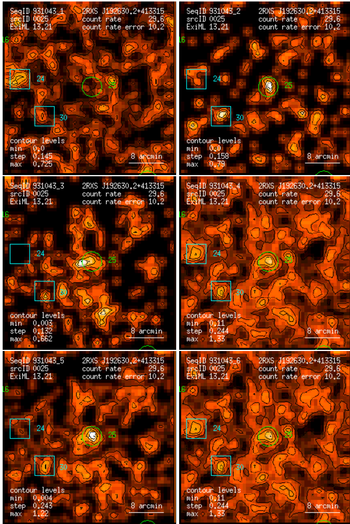
Figure 25: RASS 931043: detection 0025: band rate images, Gaussian filter: (1) PSPC channels 11 – 41, (2) 52 – 90, (3) 91 – 201, (4) 11 – 235, (5) 52 – 201, (6) 11 – 201. Broad band rates in counts/ks. Band rate contour levels in counts/ks/arcmin 2 .
