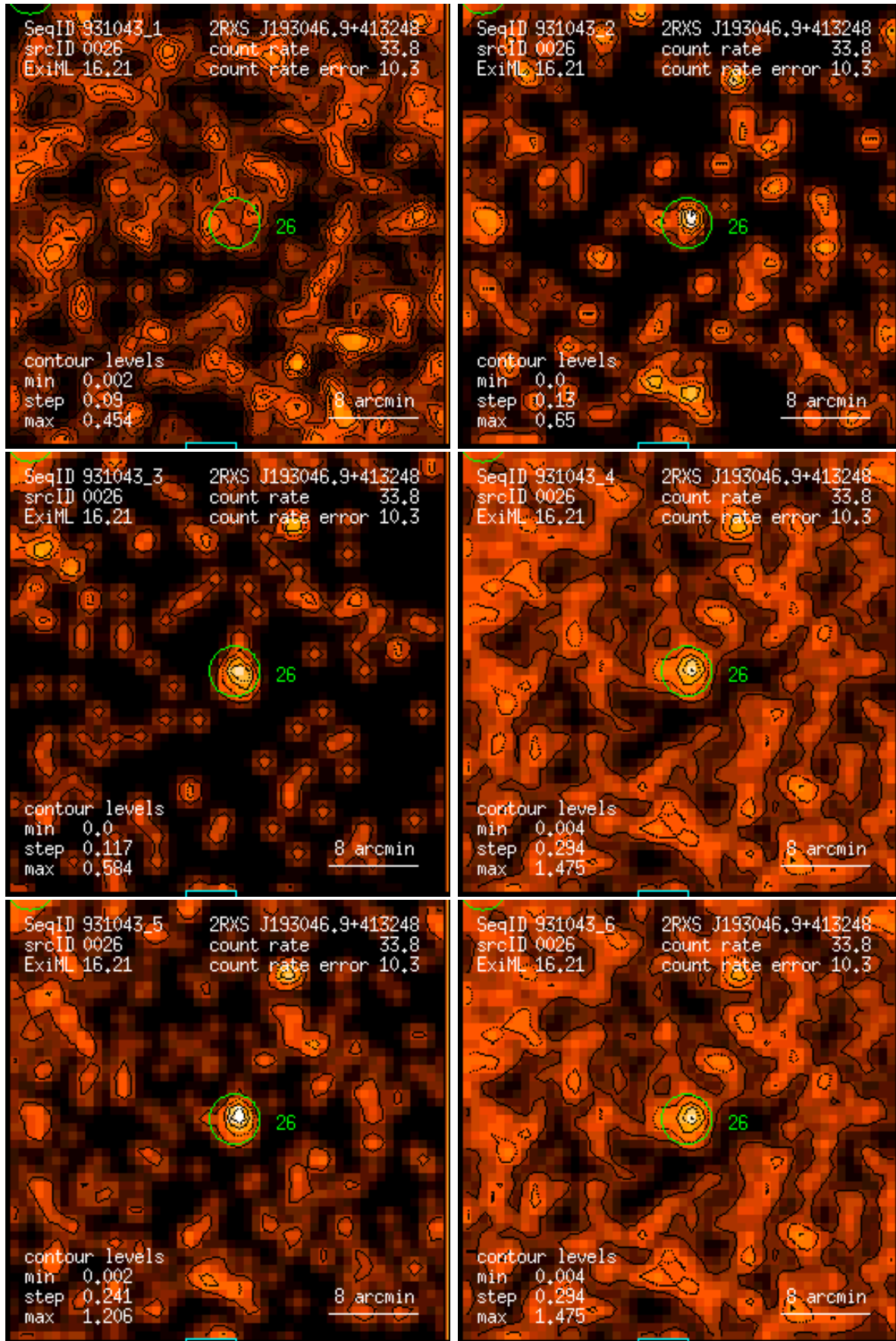
Figure 26: RASS 931043: detection 0026: band rate images, Gaussian filter: (1) PSPC channels 11 – 41, (2) 52 – 90, (3) 91 – 201, (4) 11 – 235, (5) 52 – 201, (6) 11 – 201. Broad band rates in counts/ks. Band rate contour levels in counts/ks/arcmin 2 .
