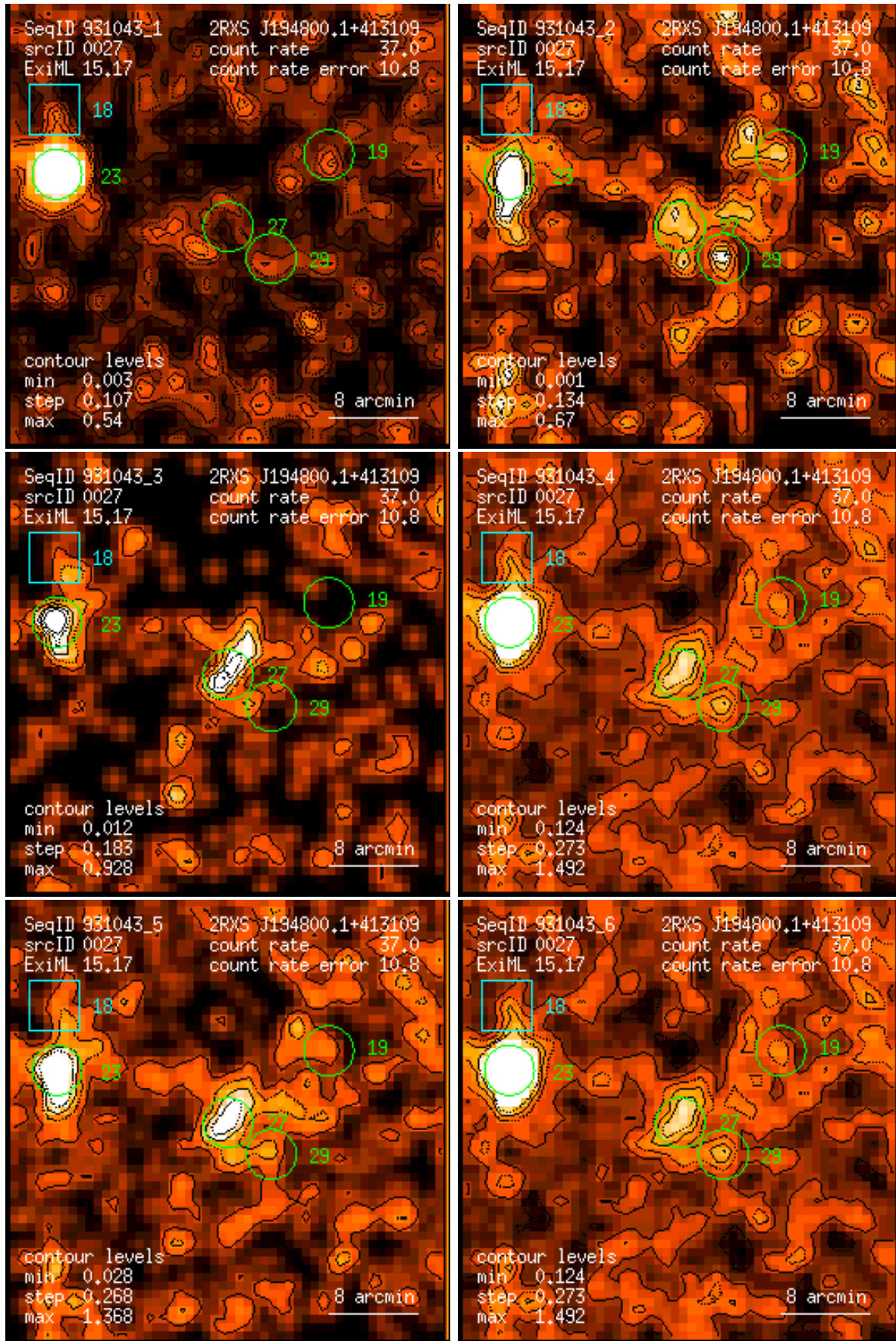
Figure 27: RASS 931043: detection 0027: band rate images, Gaussian filter: (1) PSPC channels 11 – 41, (2) 52 – 90, (3) 91 – 201, (4) 11 – 235, (5) 52 – 201, (6) 11 – 201. Broad band rates in counts/ks. Band rate contour levels in counts/ks/arcmin 2 .
