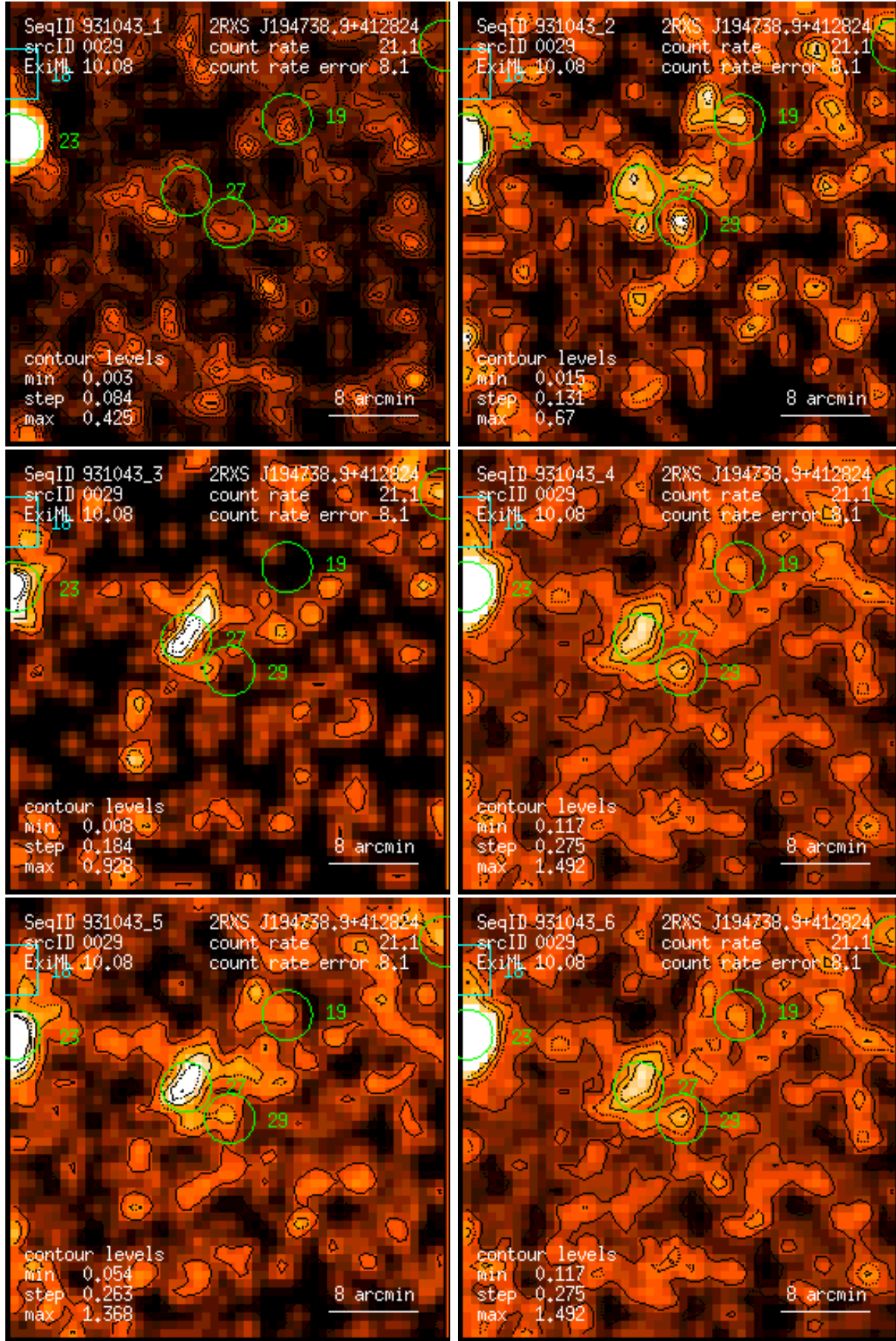
Figure 29: RASS 931043: detection 0029: band rate images, Gaussian filter: (1) PSPC channels 11 – 41, (2) 52 – 90, (3) 91 – 201, (4) 11 – 235, (5) 52 – 201, (6) 11 – 201. Broad band rates in counts/ks. Band rate contour levels in counts/ks/arcmin 2 .
