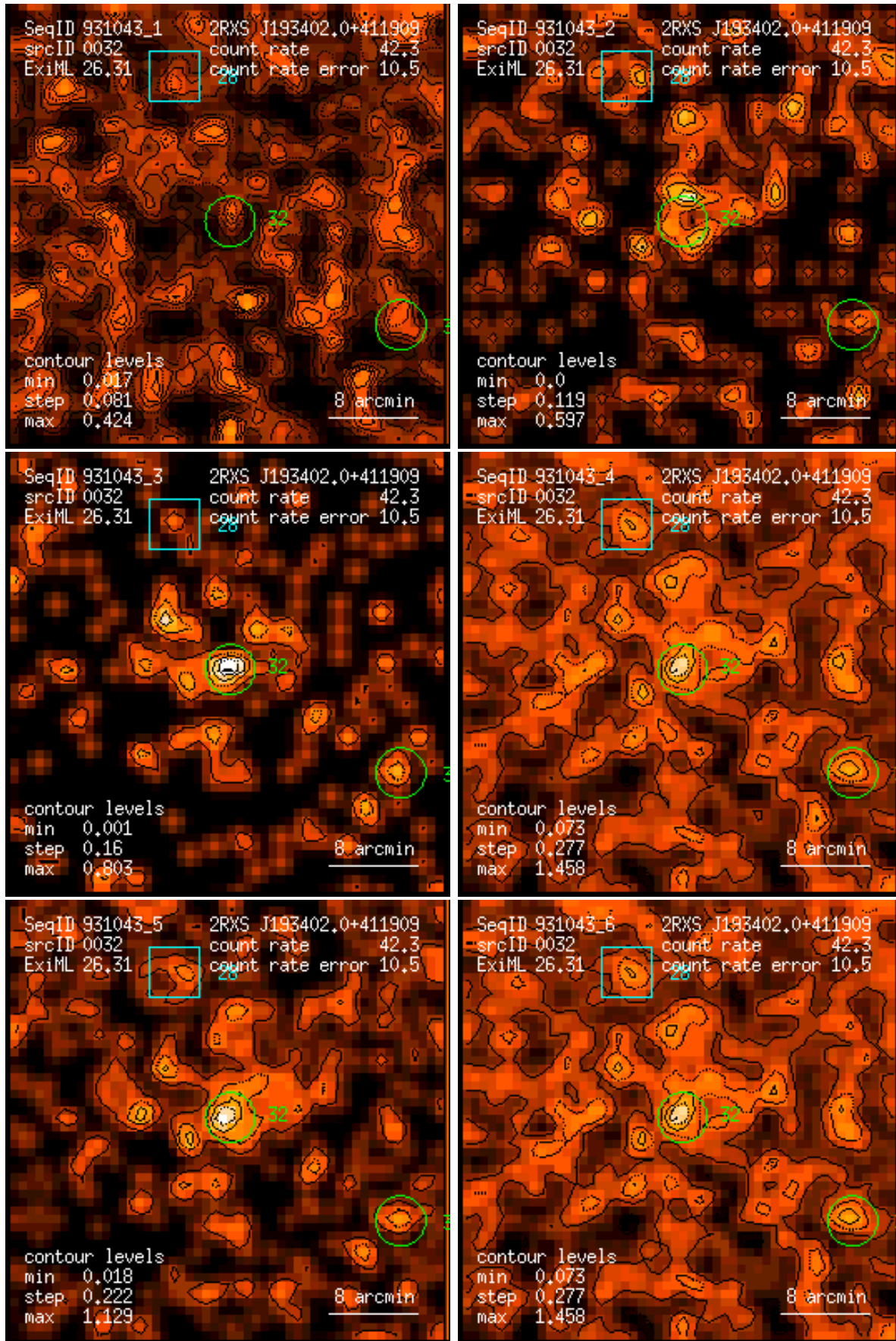
Figure 32: RASS 931043: detection 0032: band rate images, Gaussian filter: (1) PSPC channels 11 – 41, (2) 52 – 90, (3) 91 – 201, (4) 11 – 235, (5) 52 – 201, (6) 11 – 201. Broad band rates in counts/ks. Band rate contour levels in counts/ks/arcmin 2 .
