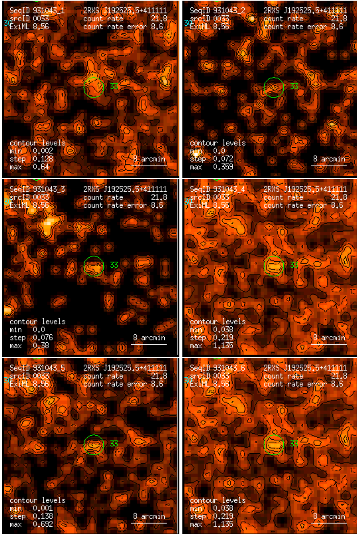
Figure 33: RASS 931043: detection 0033: band rate images, Gaussian filter: (1) PSPC channels 11 – 41, (2) 52 – 90, (3) 91 – 201, (4) 11 – 235, (5) 52 – 201, (6) 11 – 201. Broad band rates in counts/ks. Band rate contour levels in counts/ks/arcmin 2 .
