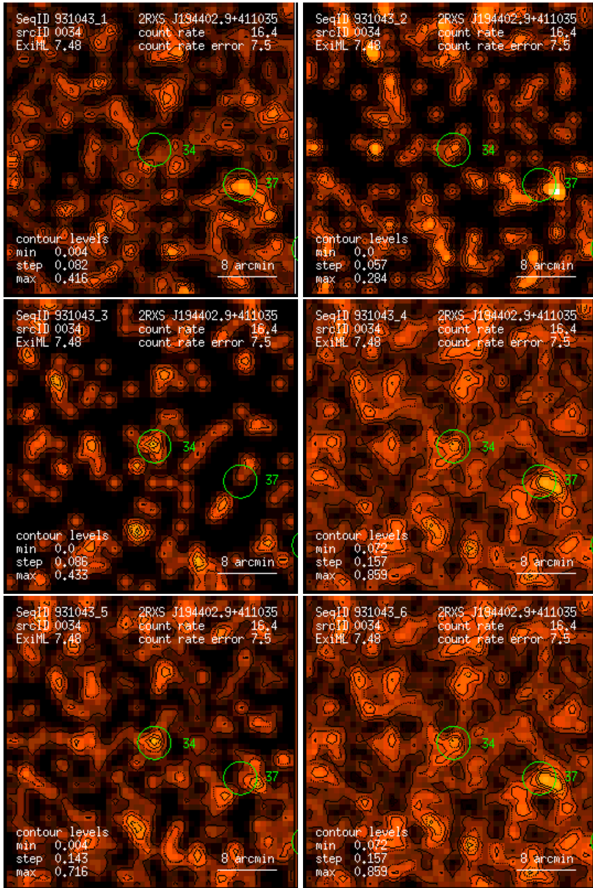
Figure 34: RASS 931043: detection 0034: band rate images, Gaussian filter: (1) PSPC channels 11 – 41, (2) 52 – 90, (3) 91 – 201, (4) 11 – 235, (5) 52 – 201, (6) 11 – 201. Broad band rates in counts/ks. Band rate contour levels in counts/ks/arcmin 2 .
