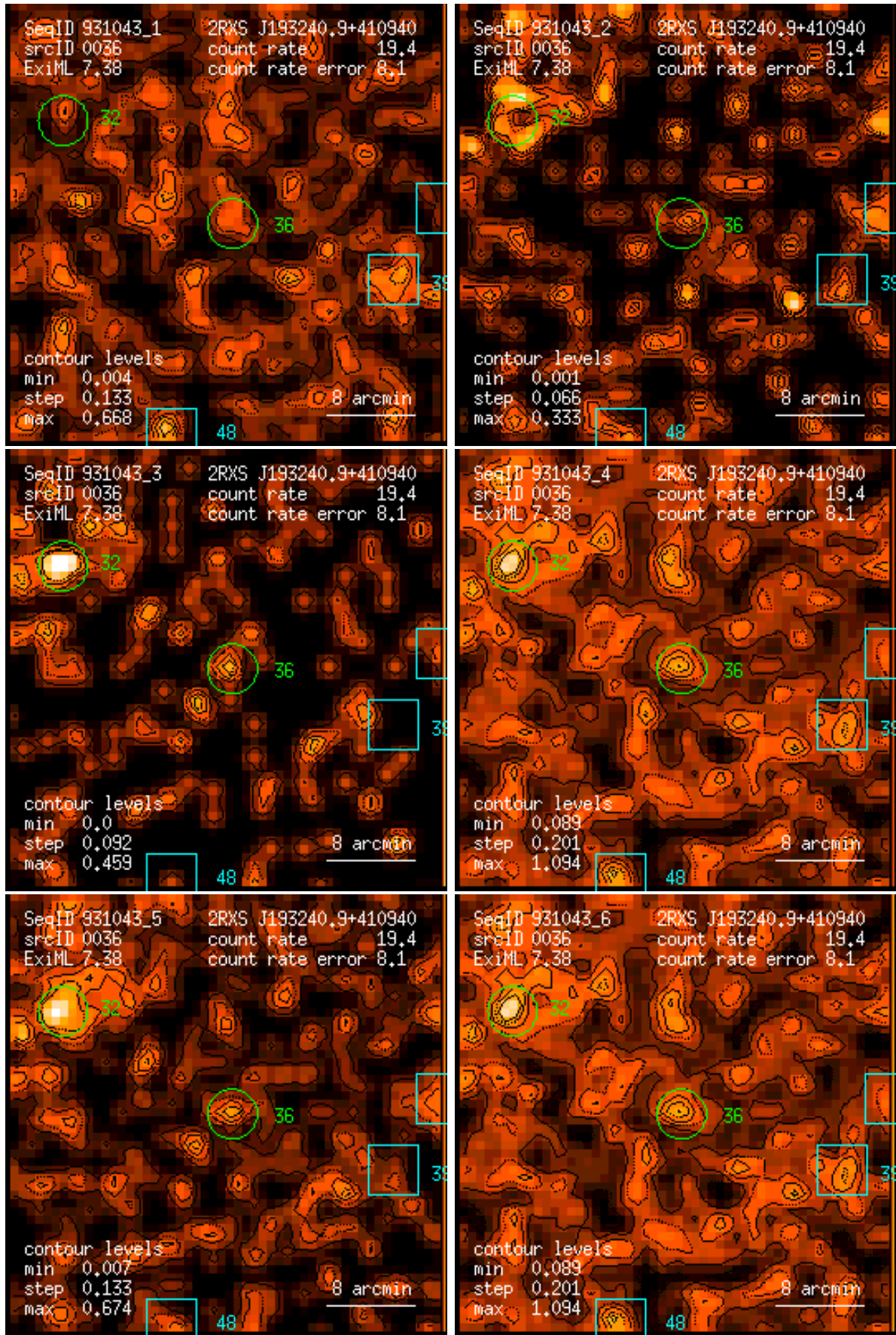
Figure 36: RASS 931043: detection 0036: band rate images, Gaussian filter: (1) PSPC channels 11 – 41, (2) 52 – 90, (3) 91 – 201, (4) 11 – 235, (5) 52 – 201, (6) 11 – 201. Broad band rates in counts/ks. Band rate contour levels in counts/ks/arcmin 2 .
