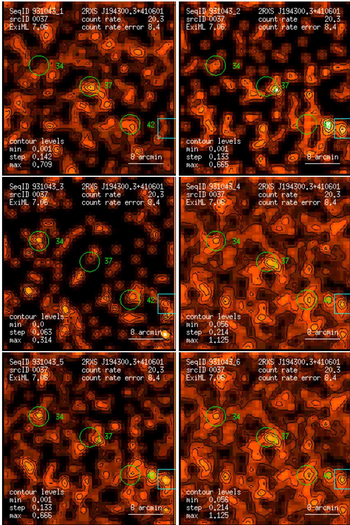
Figure 37: RASS 931043: detection 0037: band rate images, Gaussian filter: (1) PSPC channels 11 – 41, (2) 52 – 90, (3) 91 – 201, (4) 11 – 235, (5) 52 – 201, (6) 11 – 201. Broad band rates in counts/ks. Band rate contour levels in counts/ks/arcmin 2 .
