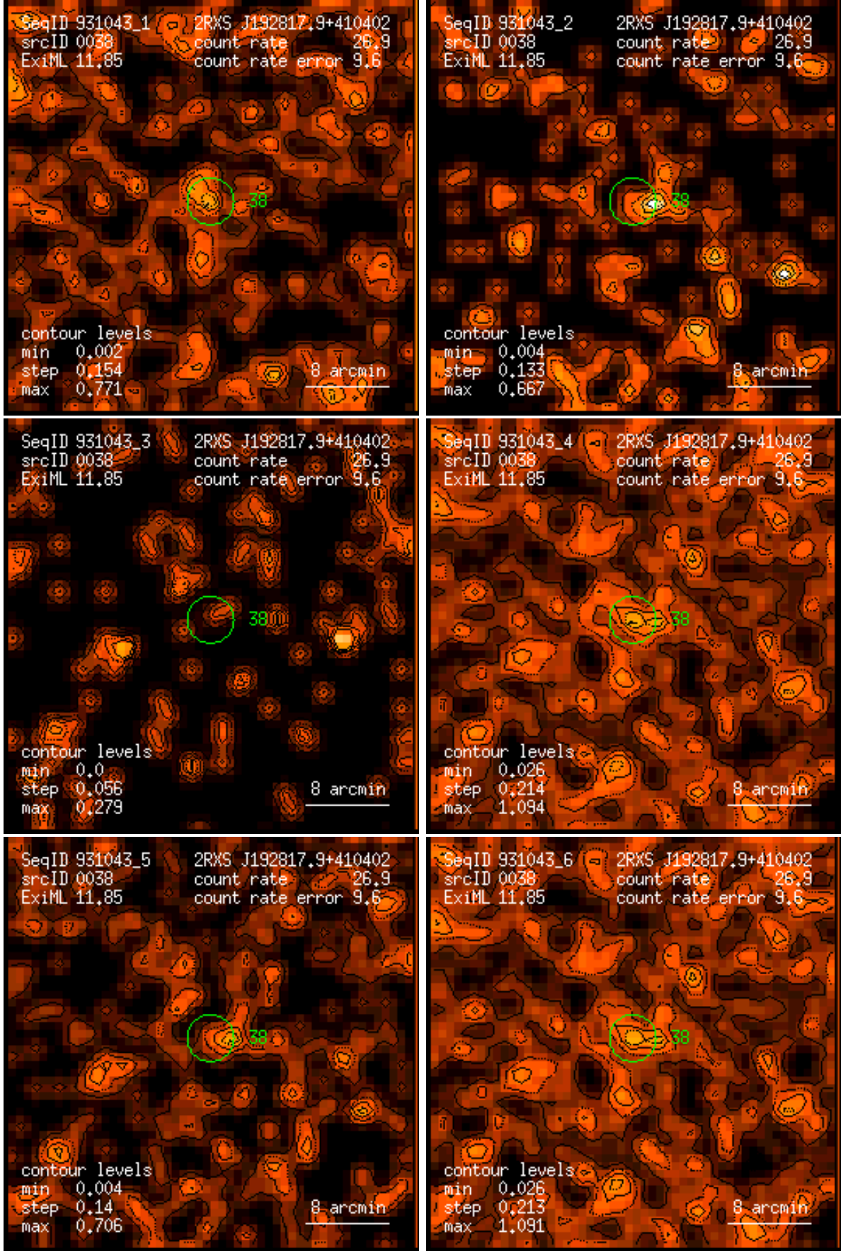
Figure 38: RASS 931043: detection 0038: band rate images, Gaussian filter: (1) PSPC channels 11 – 41, (2) 52 – 90, (3) 91 – 201, (4) 11 – 235, (5) 52 – 201, (6) 11 – 201. Broad band rates in counts/ks. Band rate contour levels in counts/ks/arcmin 2 .
