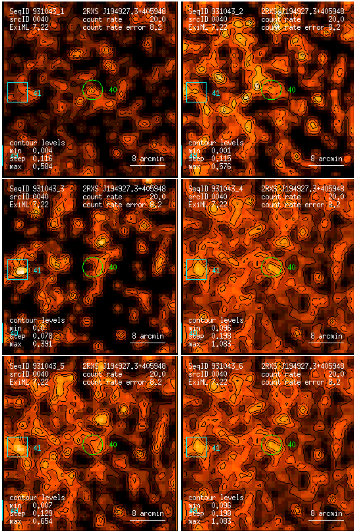
Figure 40: RASS 931043: detection 0040: band rate images, Gaussian filter: (1) PSPC channels 11 – 41, (2) 52 – 90, (3) 91 – 201, (4) 11 – 235, (5) 52 – 201, (6) 11 – 201. Broad band rates in counts/ks. Band rate contour levels in counts/ks/arcmin 2 .
