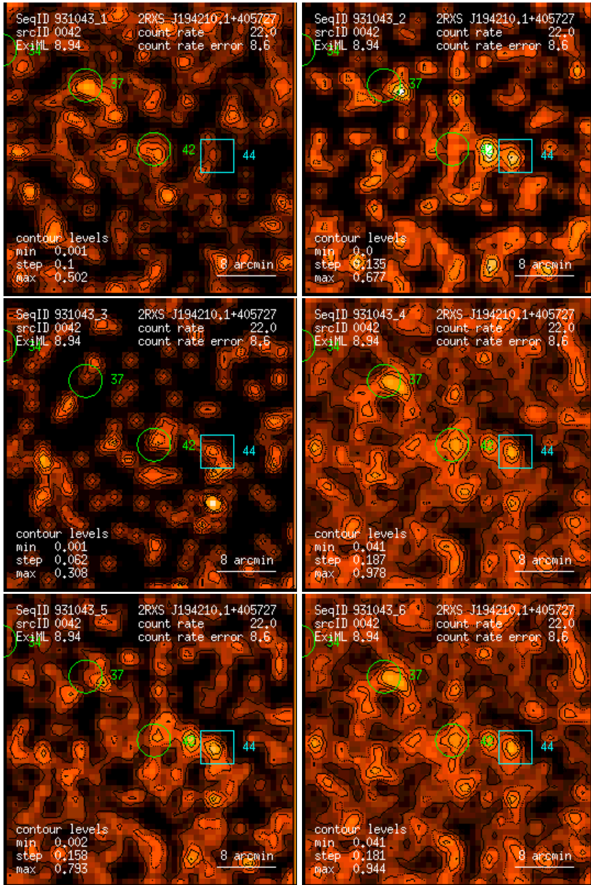
Figure 42: RASS 931043: detection 0042: band rate images, Gaussian filter: (1) PSPC channels 11 – 41, (2) 52 – 90, (3) 91 – 201, (4) 11 – 235, (5) 52 – 201, (6) 11 – 201. Broad band rates in counts/ks. Band rate contour levels in counts/ks/arcmin 2 .
