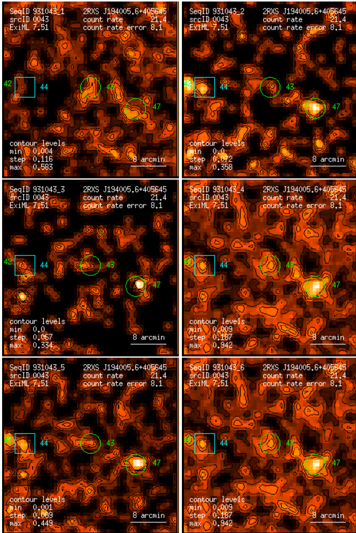
Figure 43: RASS 931043: detection 0043: band rate images, Gaussian filter: (1) PSPC channels 11 – 41, (2) 52 – 90, (3) 91 – 201, (4) 11 – 235, (5) 52 – 201, (6) 11 – 201. Broad band rates in counts/ks. Band rate contour levels in counts/ks/arcmin 2 .
