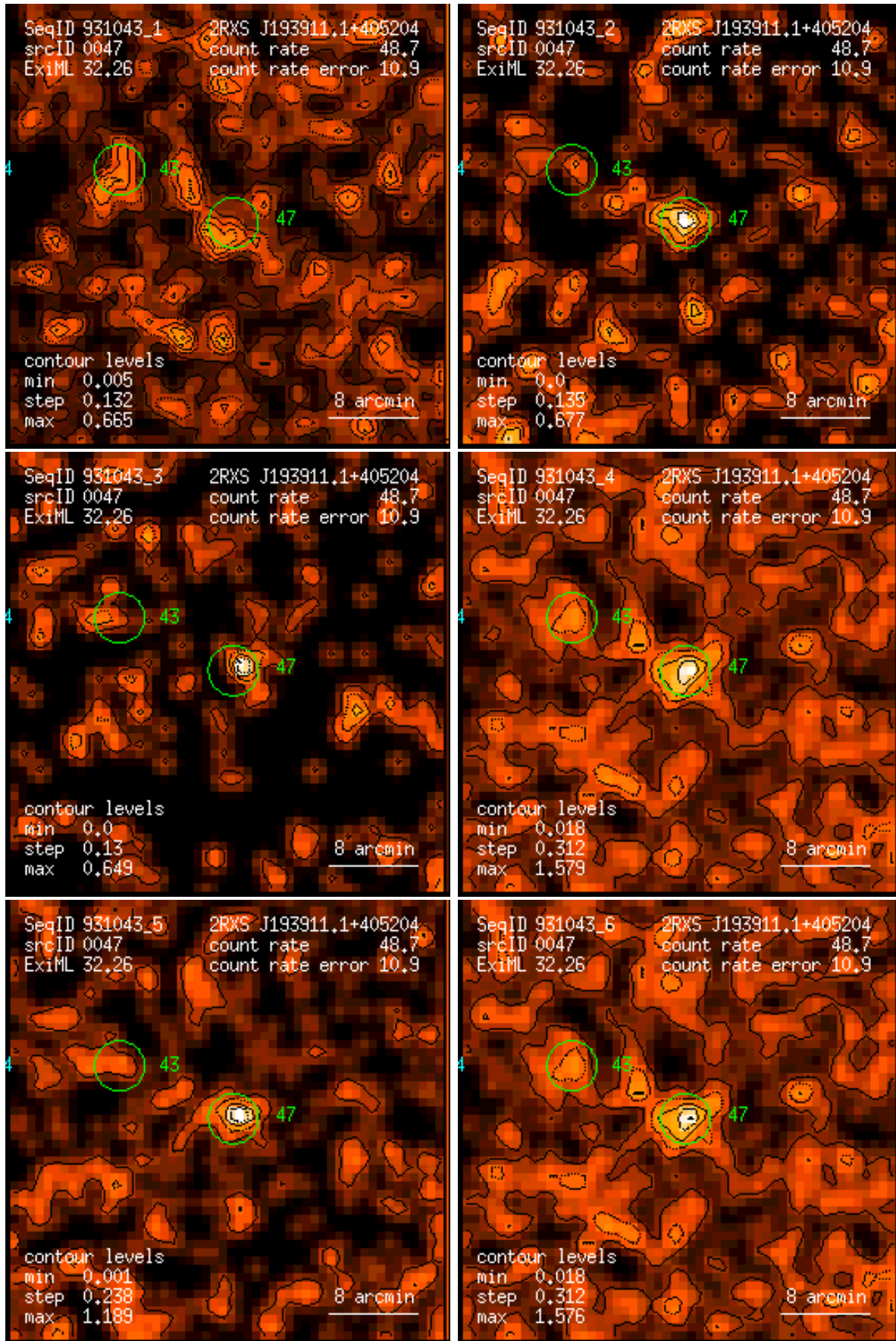
Figure 47: RASS 931043: detection 0047: band rate images, Gaussian filter: (1) PSPC channels 11 – 41, (2) 52 – 90, (3) 91 – 201, (4) 11 – 235, (5) 52 – 201, (6) 11 – 201. Broad band rates in counts/ks. Band rate contour levels in counts/ks/arcmin 2 .
