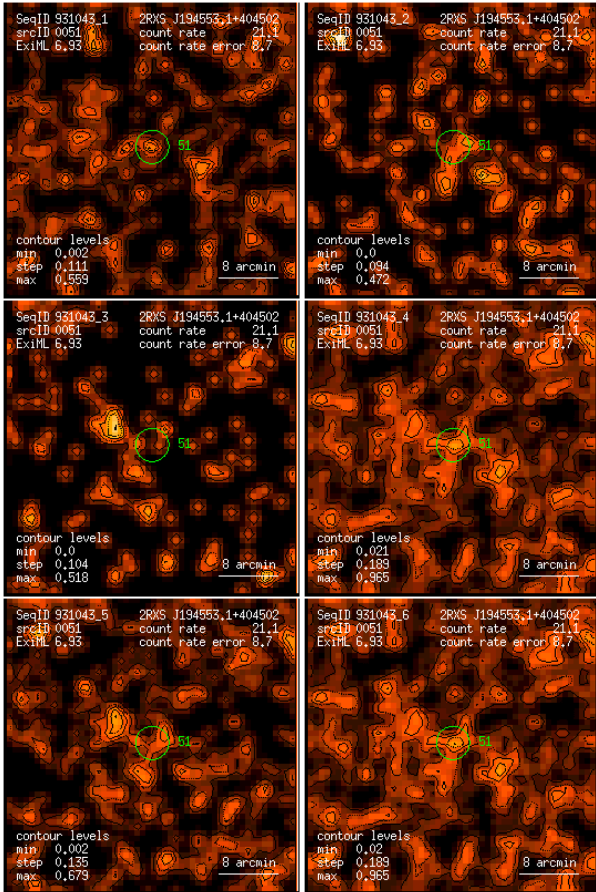
Figure 51: RASS 931043: detection 0051: band rate images, Gaussian filter: (1) PSPC channels 11 – 41, (2) 52 – 90, (3) 91 – 201, (4) 11 – 235, (5) 52 – 201, (6) 11 – 201. Broad band rates in counts/ks. Band rate contour levels in counts/ks/arcmin 2 .
