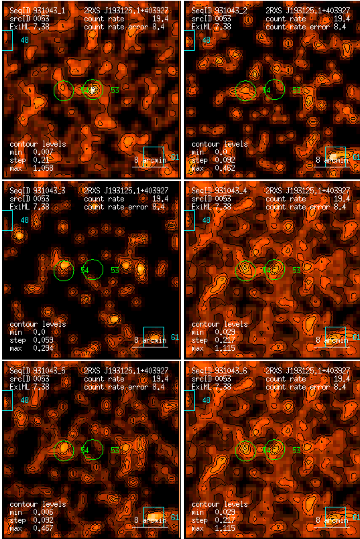
Figure 53: RASS 931043: detection 0053: band rate images, Gaussian filter: (1) PSPC channels 11 – 41, (2) 52 – 90, (3) 91 – 201, (4) 11 – 235, (5) 52 – 201, (6) 11 – 201. Broad band rates in counts/ks. Band rate contour levels in counts/ks/arcmin 2 .
