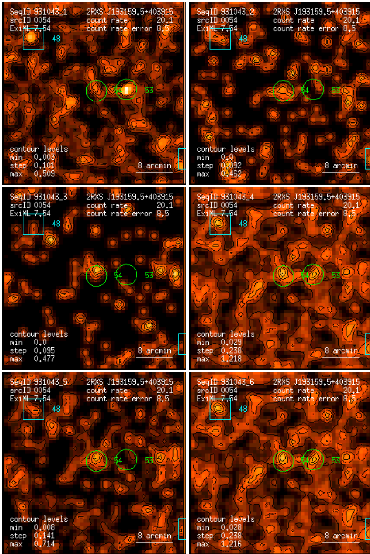
Figure 54: RASS 931043: detection 0054: band rate images, Gaussian filter: (1) PSPC channels 11 – 41, (2) 52 – 90, (3) 91 – 201, (4) 11 – 235, (5) 52 – 201, (6) 11 – 201. Broad band rates in counts/ks. Band rate contour levels in counts/ks/arcmin 2 .
