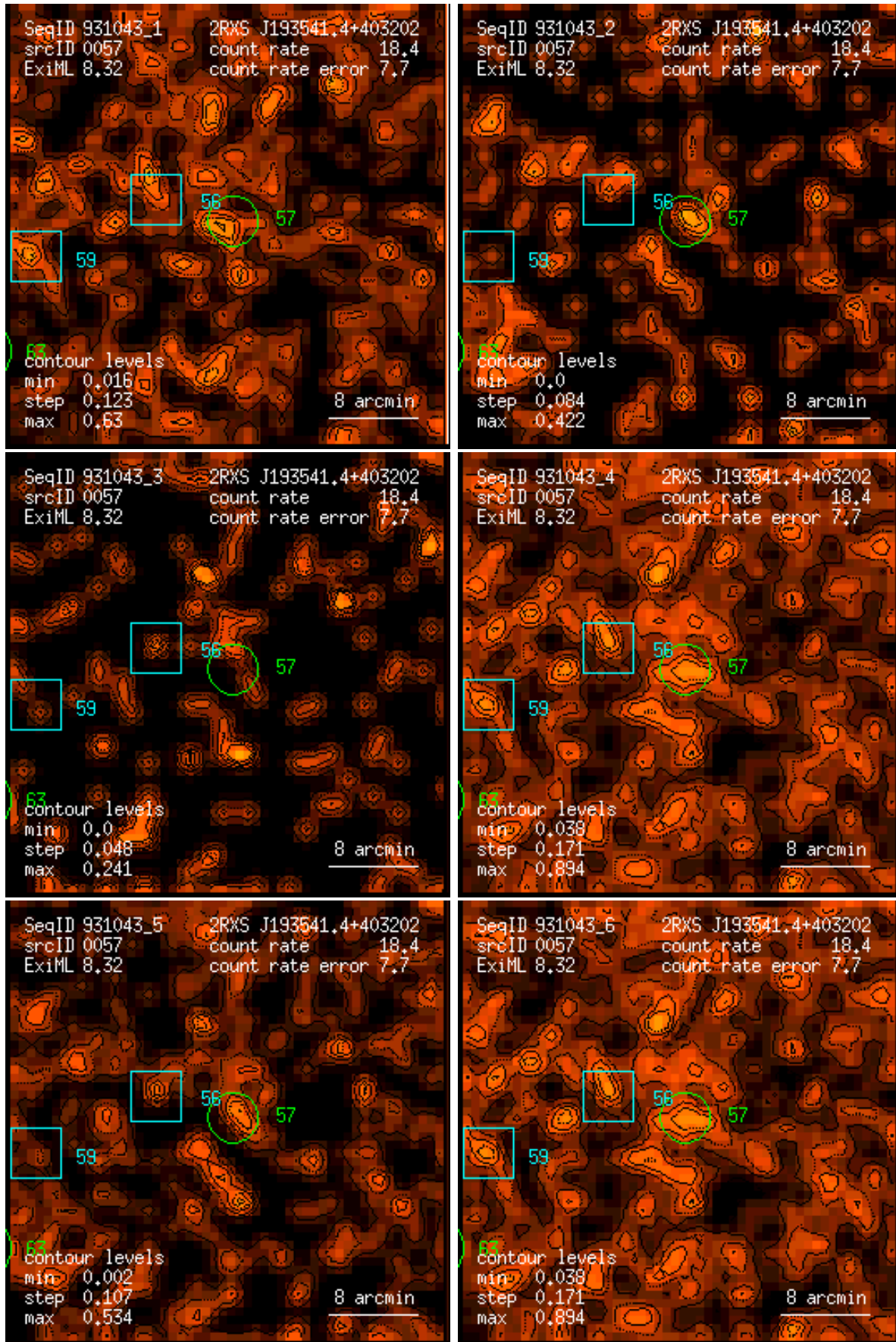
Figure 57: RASS 931043: detection 0057: band rate images, Gaussian filter: (1) PSPC channels 11 – 41, (2) 52 – 90, (3) 91 – 201, (4) 11 – 235, (5) 52 – 201, (6) 11 – 201. Broad band rates in counts/ks. Band rate contour levels in counts/ks/arcmin 2 .
