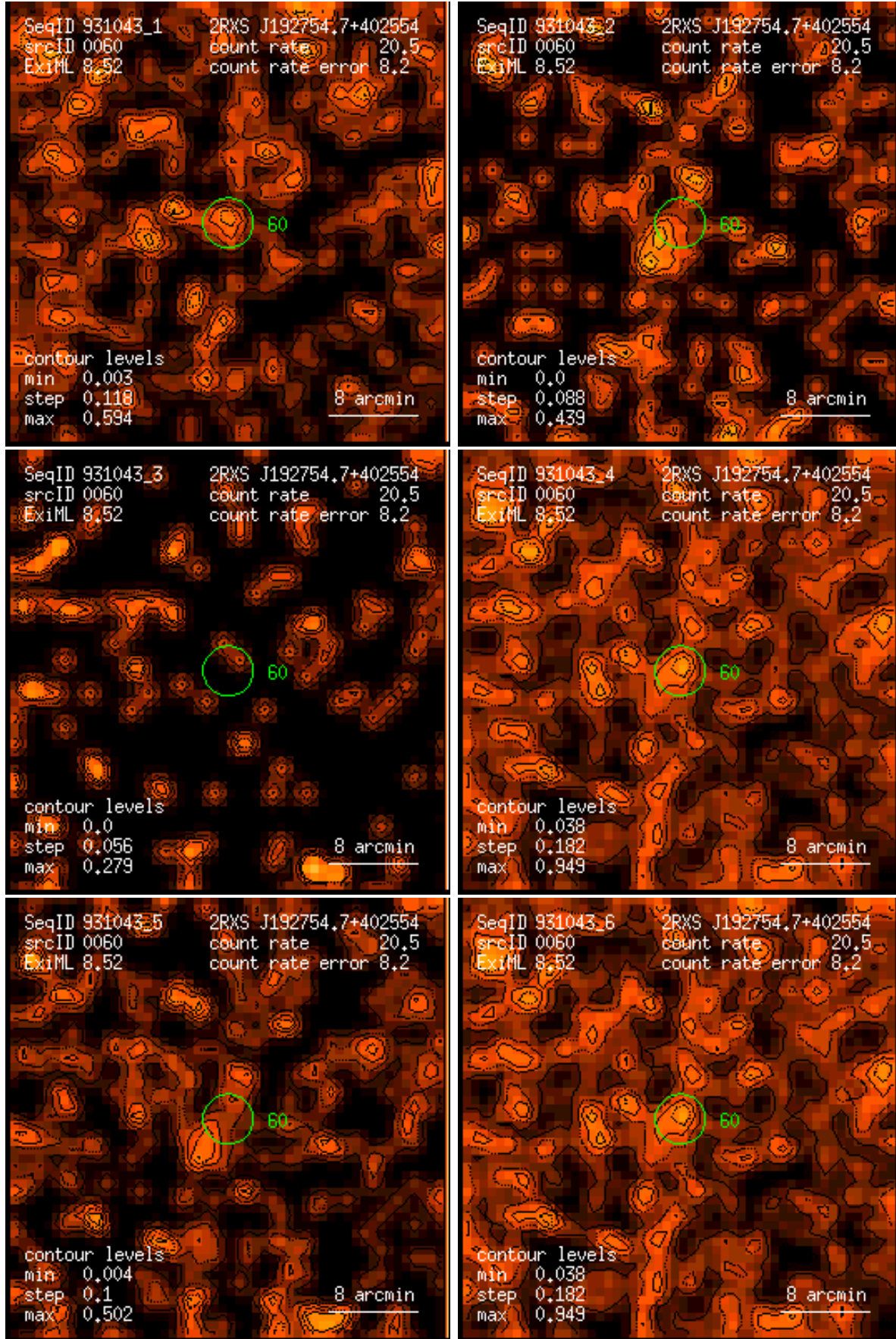
Figure 60: RASS 931043: detection 0060: band rate images, Gaussian filter: (1) PSPC channels 11 – 41, (2) 52 – 90, (3) 91 – 201, (4) 11 – 235, (5) 52 – 201, (6) 11 – 201. Broad band rates in counts/ks. Band rate contour levels in counts/ks/arcmin 2 .
